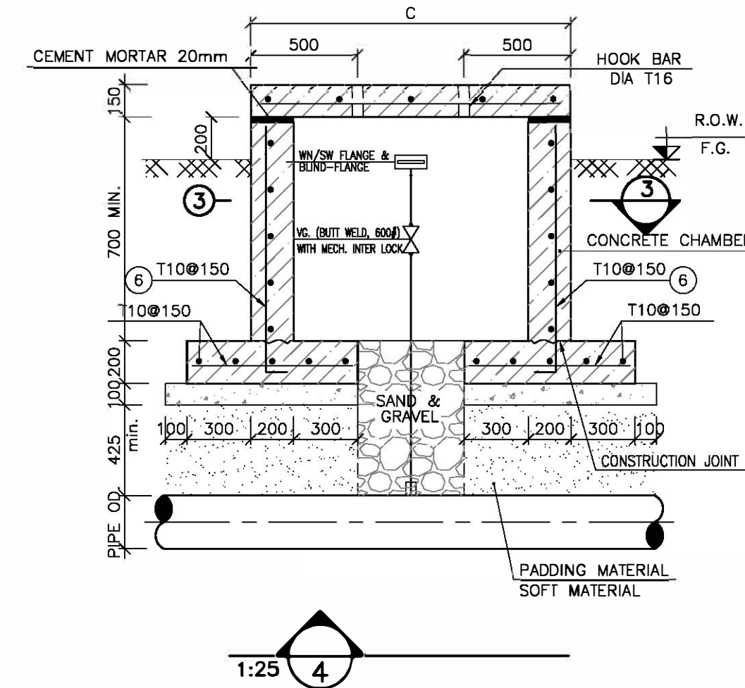
1:25 4 FOUNDATION REINFORCEMENT PLAN
