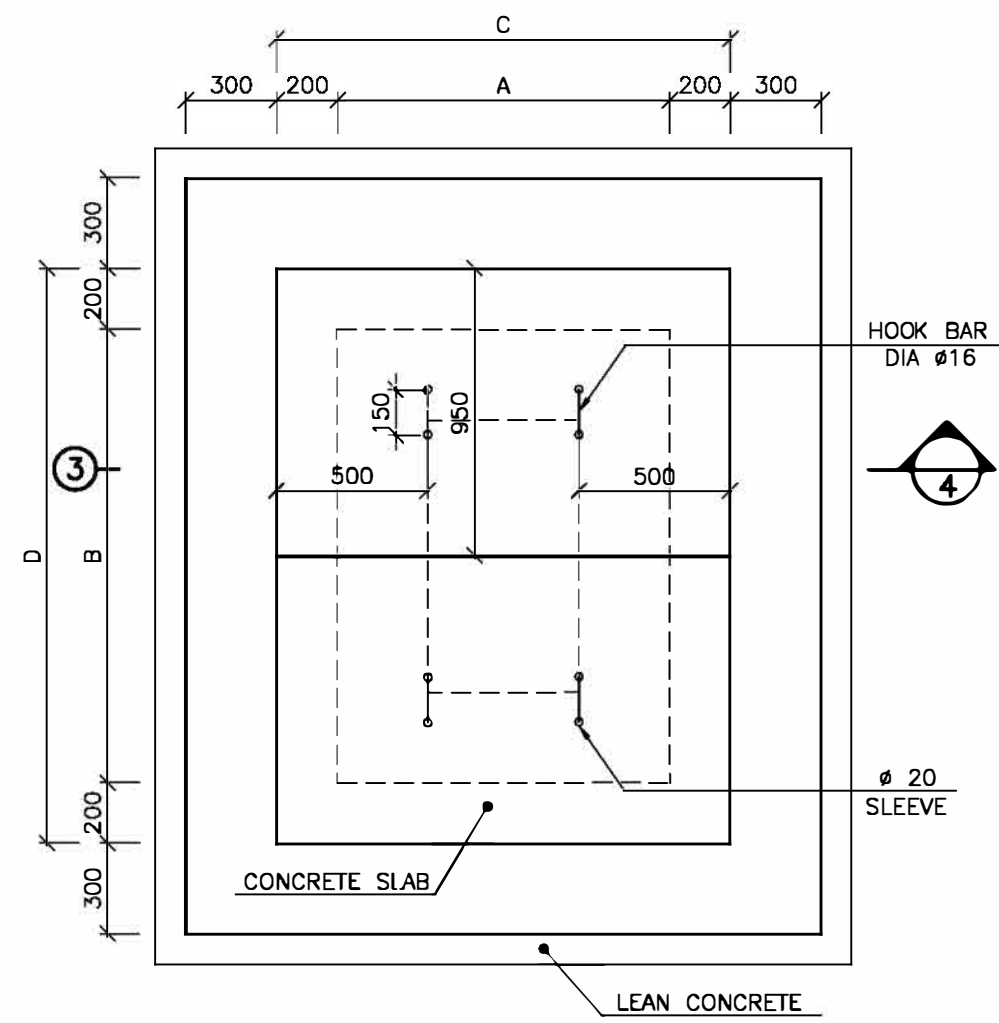
1:25 1 VALVE BOX FORMWORK PLAN
