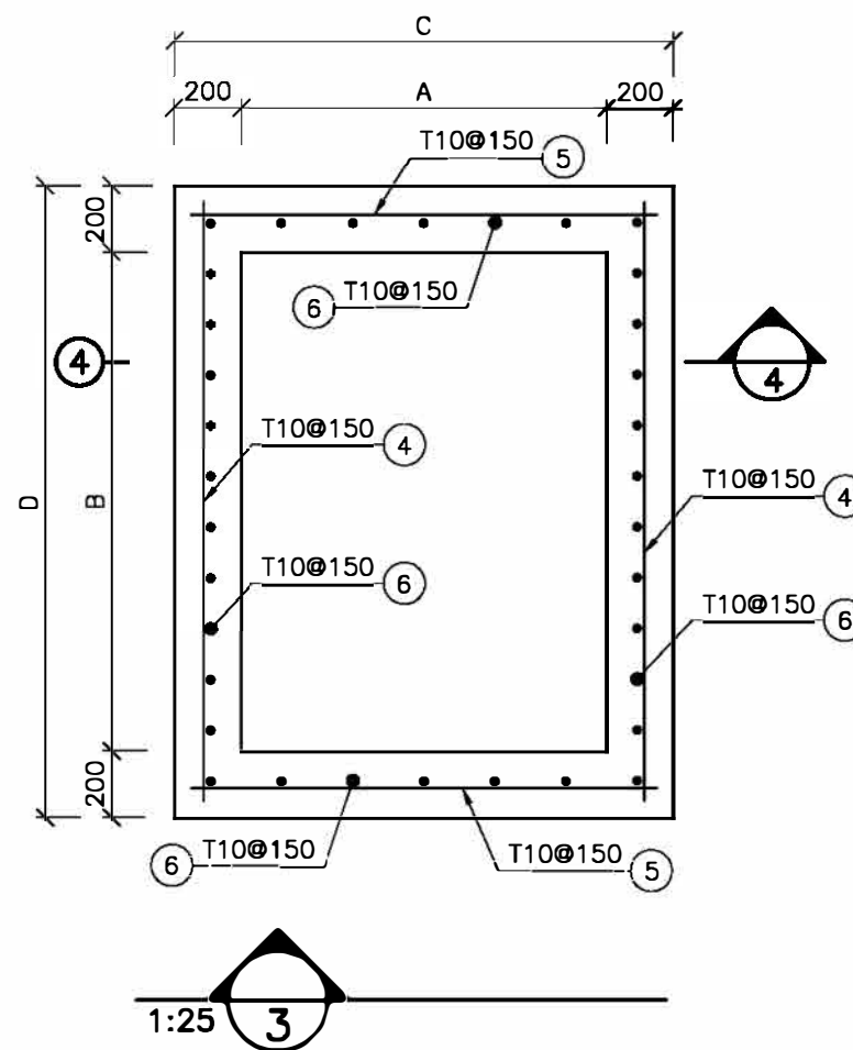
1:25 3 FOUNDATION REINFORCEMENT PLAN
