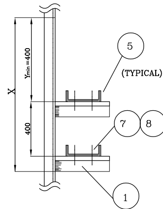
SUPPORT TO STEEL COLUMN
