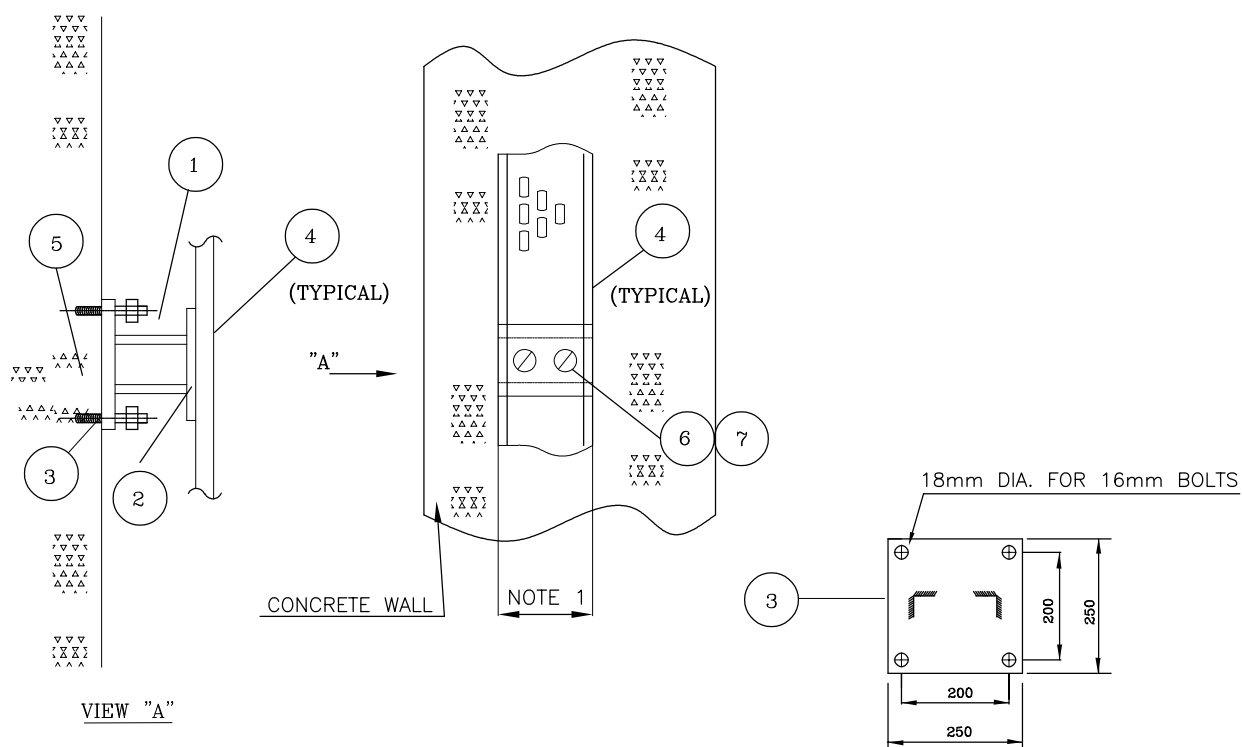
SUPPORT TO CONCRETE WALL
