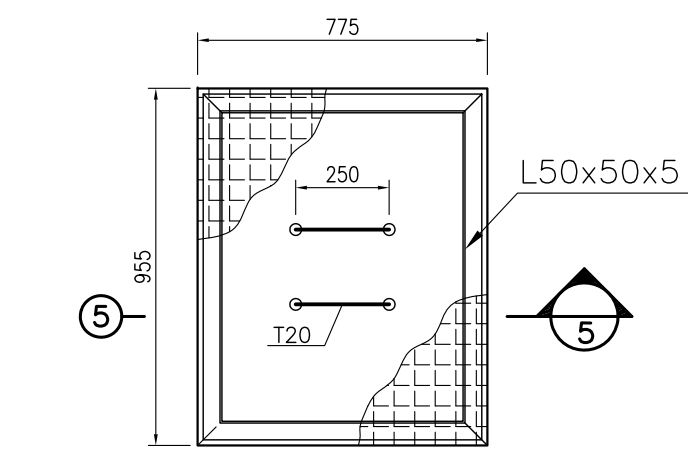
1:20 CHEQUERED PLATE
