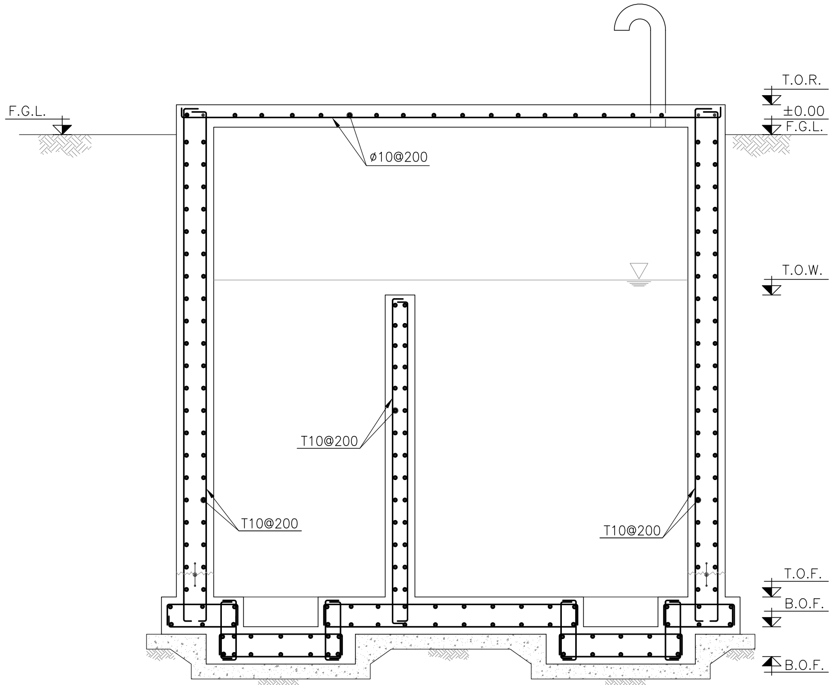
1:25 FOUNDATION PLAN REINFORCEMENT
