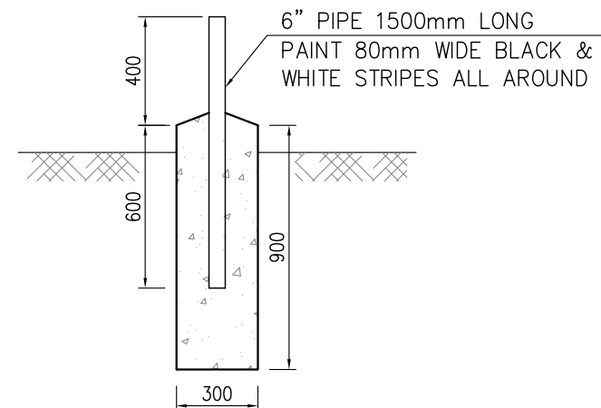
1:25 DETAIL OF MARKERS
