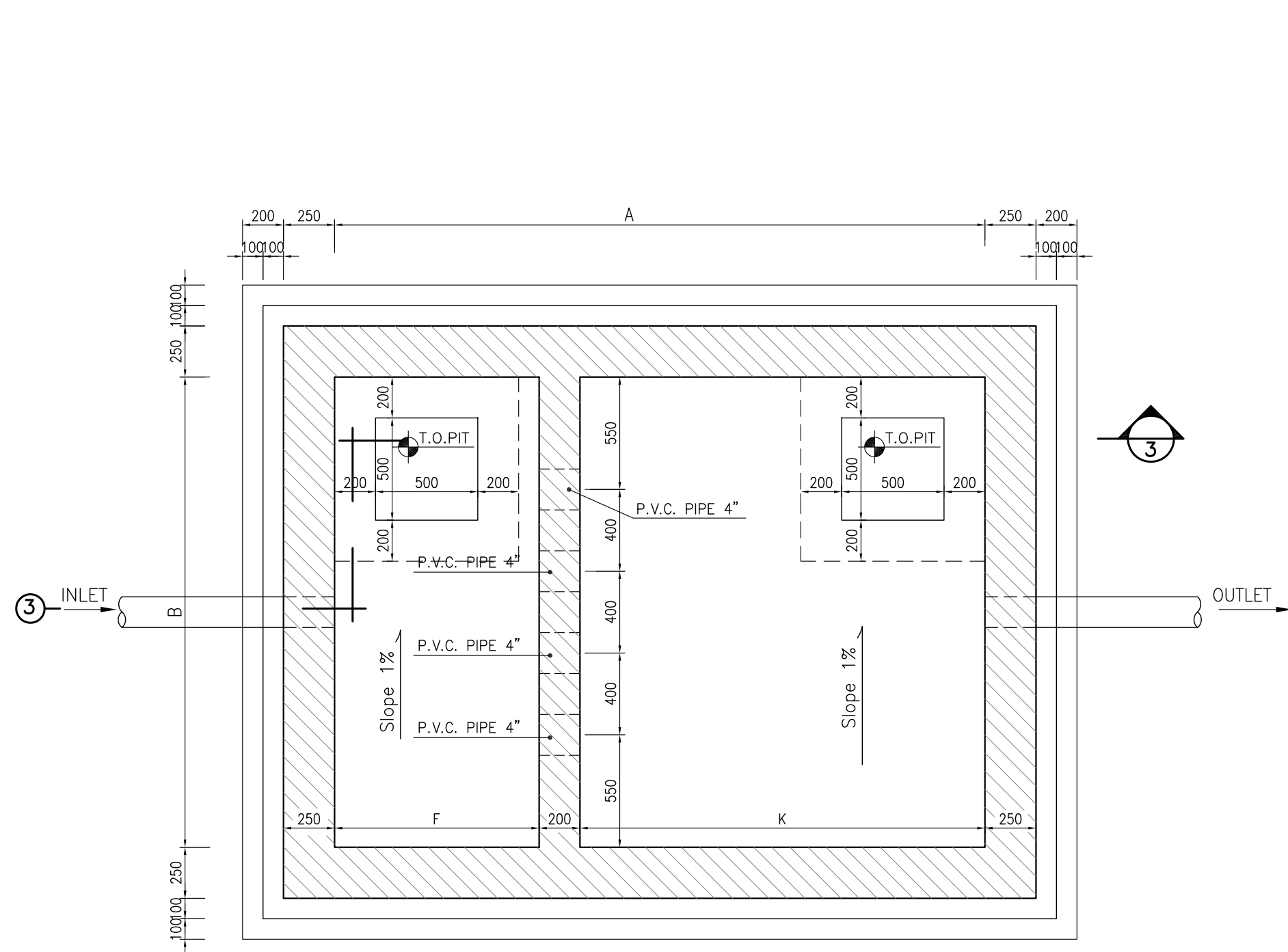
1:25 FOUNDATION PLAN SEPTIC TANK
