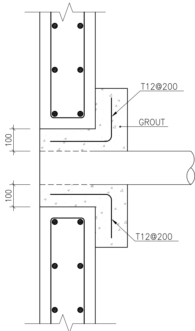
1:10 SEPTIC TANK JOIST PLAN
