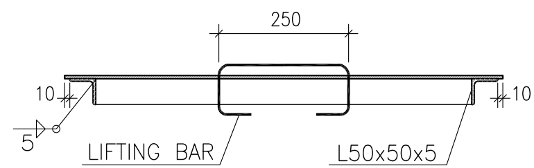
1:10 LIFTING BAR
