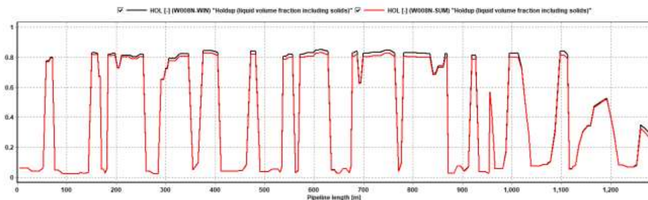
Curve 7-2.11: HOL. Profile of 6" Asmari W008N Flow Line in winter, summer (MIN-FLOW)
