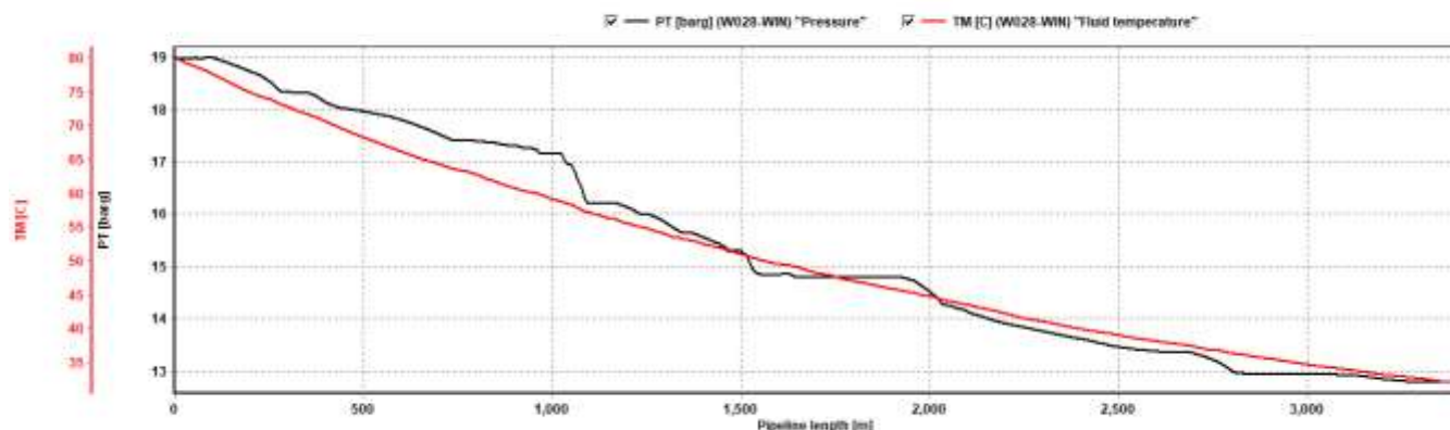
Curve 7-2.8: Temp/Press. Profile of 6" Bangestan W028 Flow Line in winter (MAX-FLOW)
