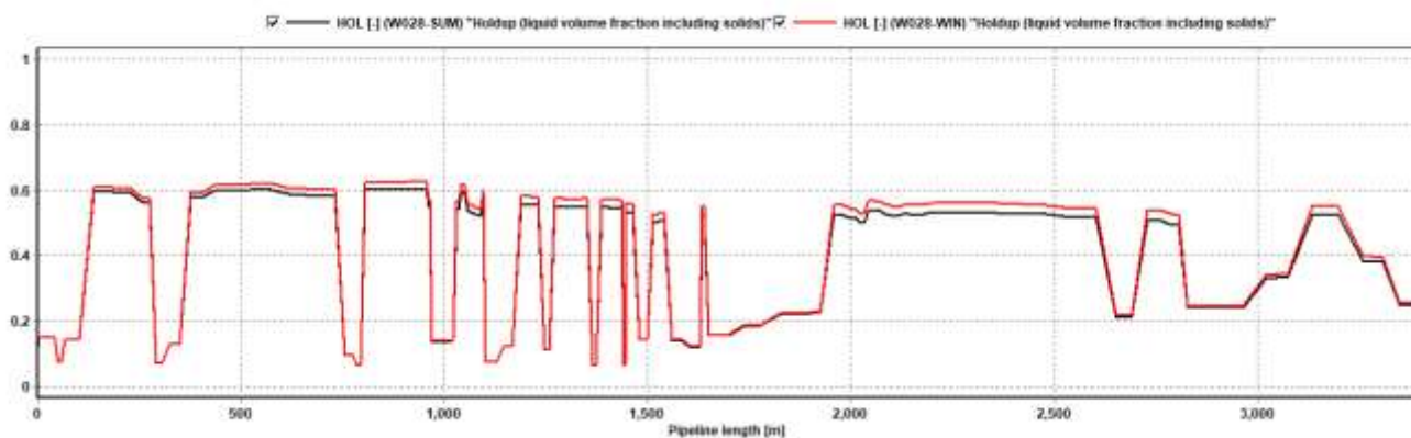
Curve 7-2.11: HOL. Profile of 6" Bangestan W028 Flow Line in Summer/Winter (MIN-FLOW)
