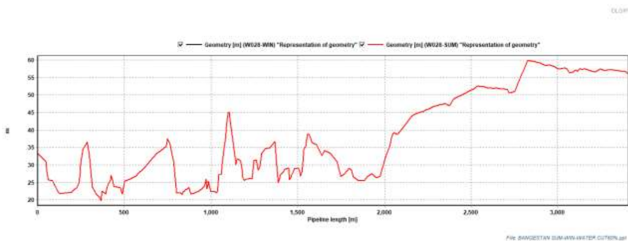
Curve 7-2.1: geometry of 6" Bangestan Flowlines
