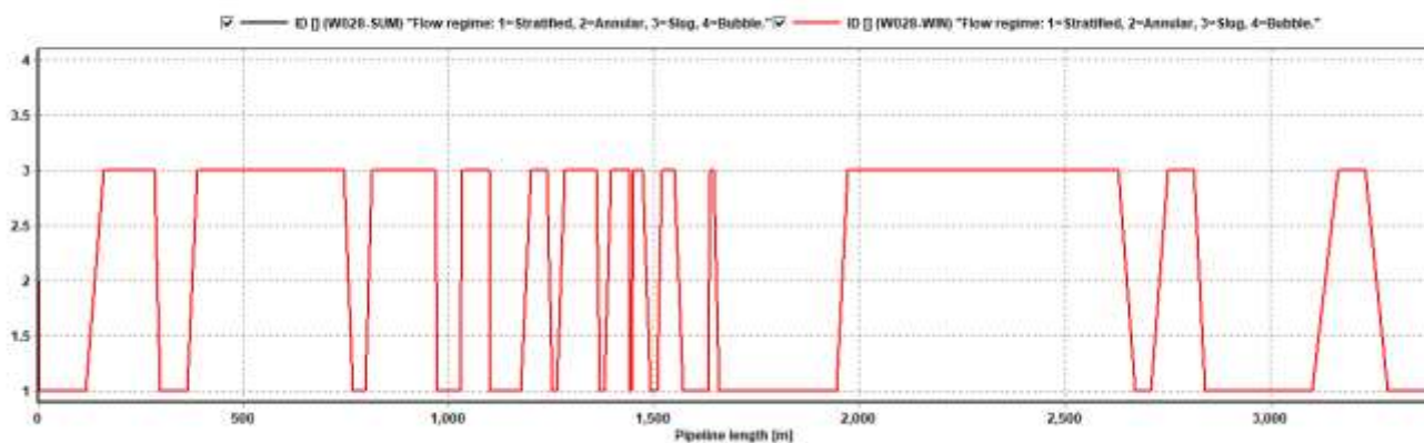
Curve 7-2.5: Flow Regime of W028 Bangestan Flowline (MIN-FLOW)
