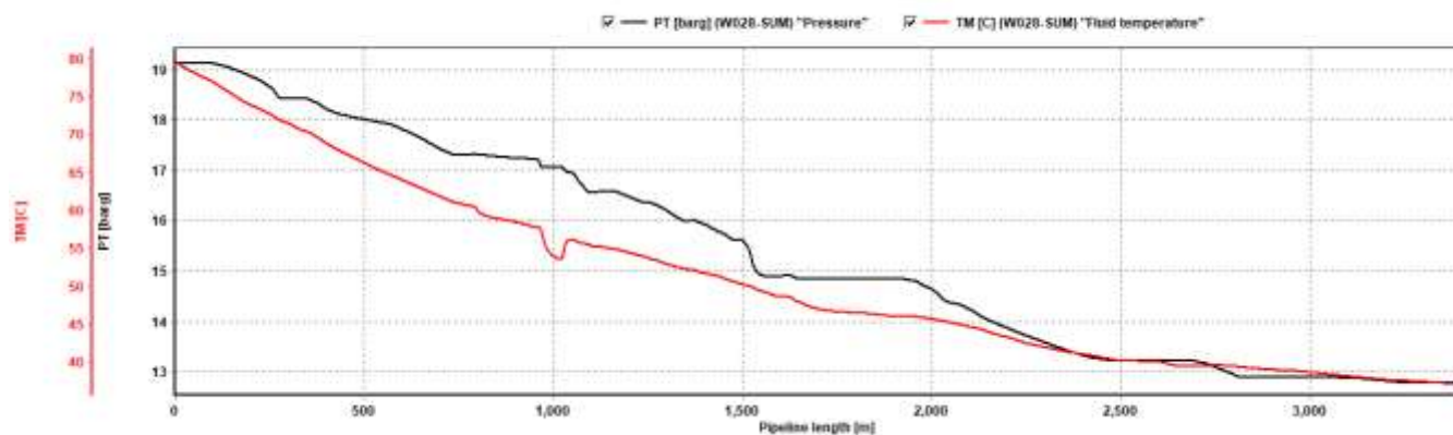
Curve 7-2.7: Temp/Press. Profile of 6" Bangestan W028 Flow Line in summer (MIN-FLOW)
