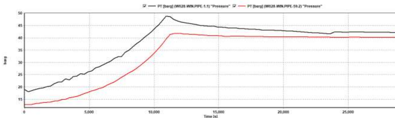
Figure 7-2.13: Surge Pressure for BANGESTAN Flow lines disposal wells (winter case)
