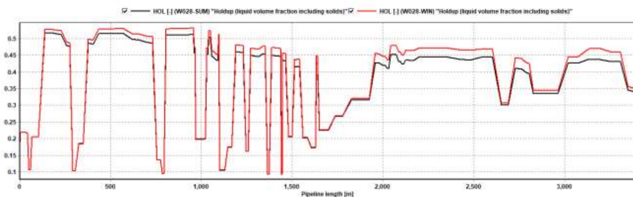
Curve 7-2.10: HOL. Profile of 6" Bangestan W028 Flow Line in Summer/Winter (Max-FLOW)
