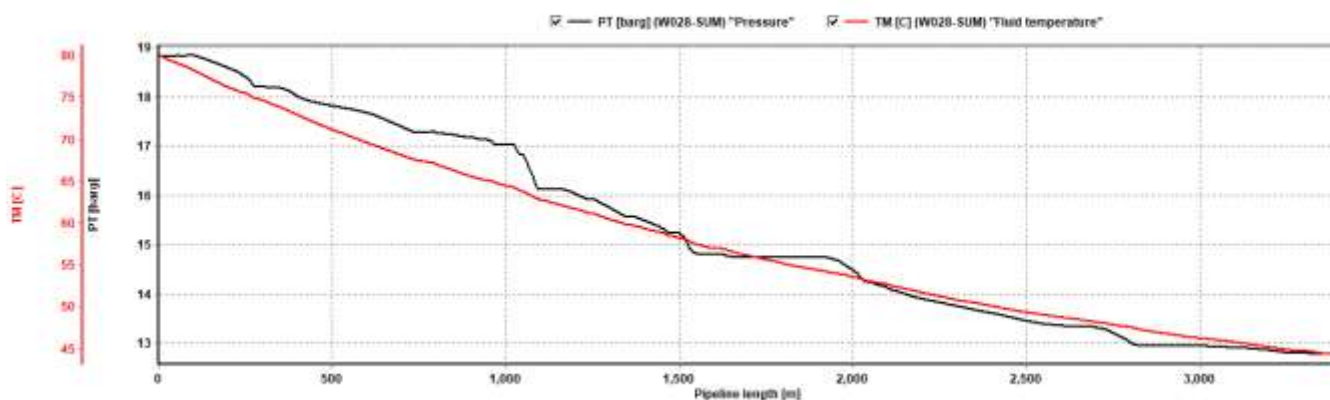
Curve 7-2.6: Temp/Press. Profile of 6" Bangestan W028 Flow Line in summer (MAX-FLOW)
