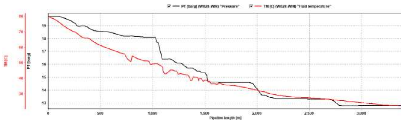
Curve 7-2.9: Temp/Press. Profile of 6" Bangestan W028 Flow Line in winter (MIN-FLOW)
