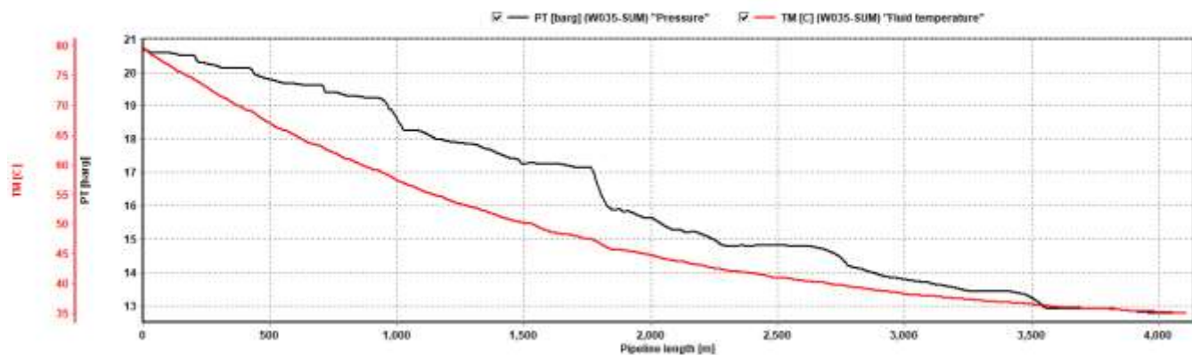
Curve 7-2.7: Temp/Press. Profile of 6" Bangestan W035 Flow Line in summer (MIN-FLOW)
