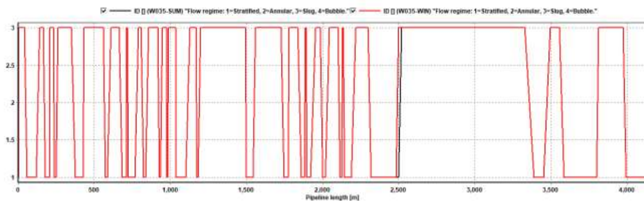
Curve 7-2.4: Flow Regime of W035 Bangestan Flowline (MAX-FLOW)
