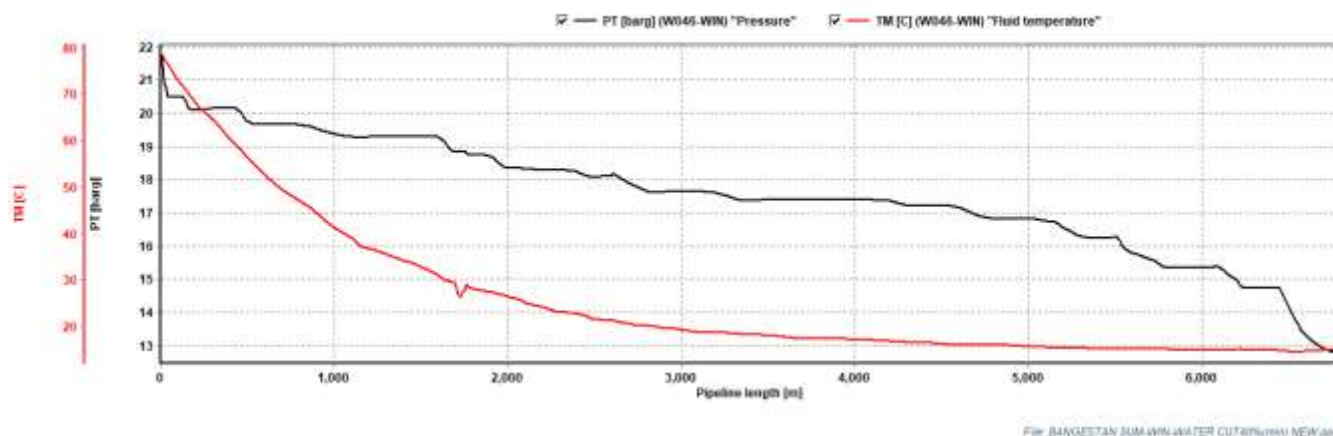
Curve 7-2.8: Temp/Press. Profile of 6" Bangestan W046S Flow Line in winter (MIN-FLOW)
