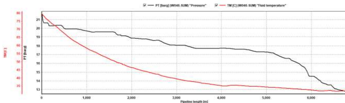
Curve 7-2.5: Temp/Press. Profile of 6" Bangestan W046S Flow Line in summer (MAX-FLOW)
