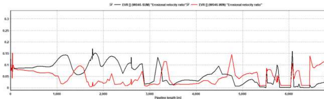
Curve 7-2.2: EVR of 6" Bangestan Flowlines in Summer& Winter (MIN-FLOW)
