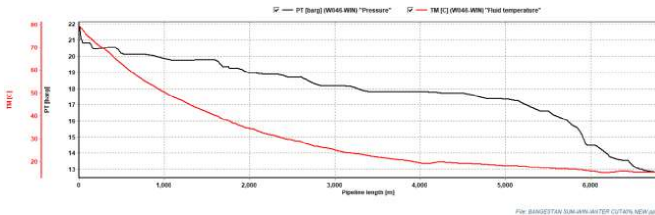
Curve 7-2.7: Temp/Press. Profile of 6" Bangestan W046S Flow Line in winter (MAX-FLOW)
