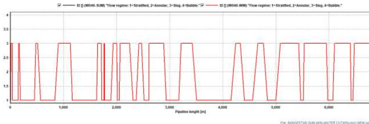
Curve 7-2.4: Flow Regime of W046 Bangestan Flowline (MIN-FLOW)
