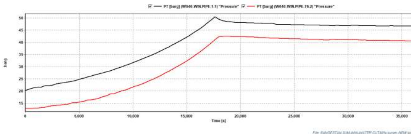
Figure 7-2.12: Surge Pressure for BANGESTAN Flow lines disposal wells (winter case/max-flow)
