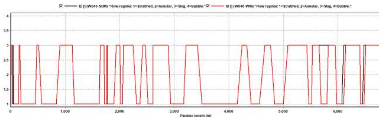
Curve 7-2.3: Flow Regime of W046 Bangestan Flowline (MAX-FLOW)
