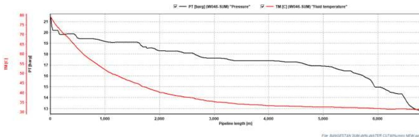
Curve 7-2.6: Temp/Press. Profile of 6" Bangestan W046S Flow Line in summer (MIN-FLOW)
