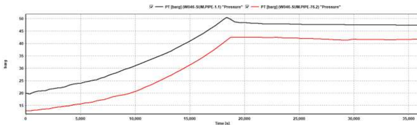
Figure 7-2.11: Surge Pressure for BANGESTAN Flow lines disposal wells (summer case/ max-flow)
