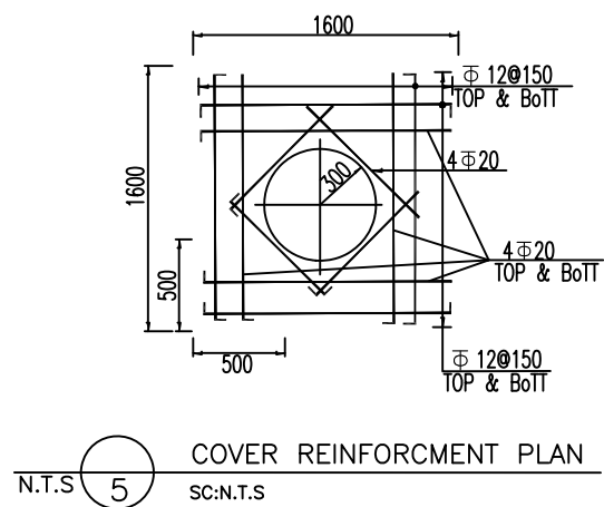
N.T.S 5 COVER REINFORCEMENT PLAN SC:N.T.S
