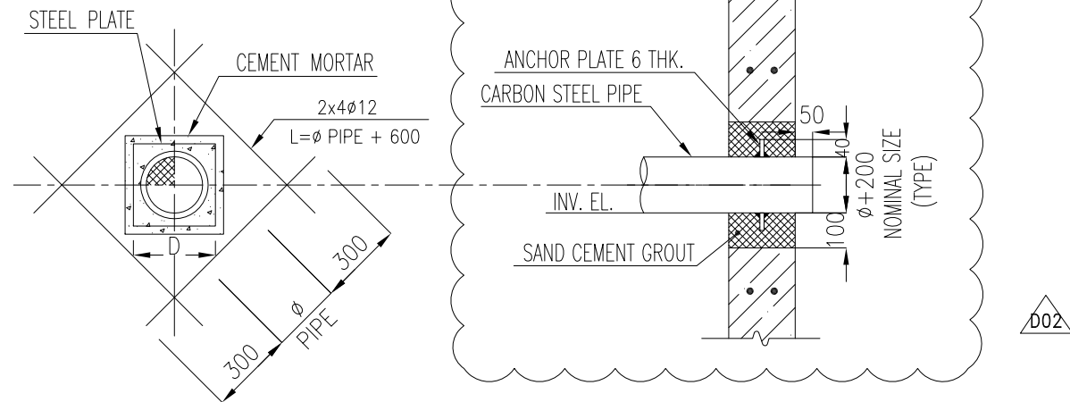
N.T.S 3 HOLES REINFORCEMENT (TYPICAL FOR INLET/OUTLET PIPE)
