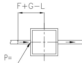
N.T.S 3 HOLES REINFORCEMENT (TYPICAL FOR INLET/OUTLET PIPE)
