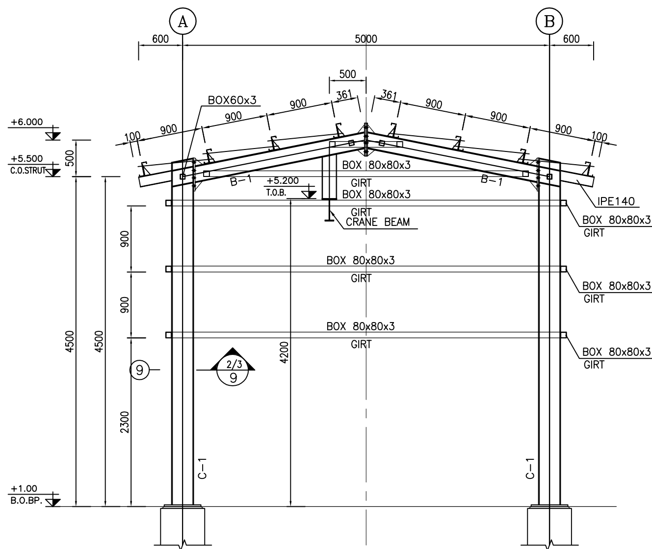
1:50 7 FRAMING ELEVATION ON AXIS 1
