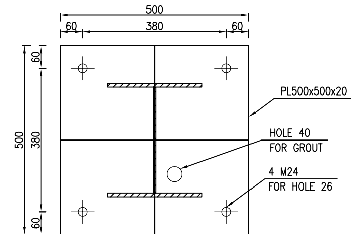
1:10 5 BASEPLATE 1 No.8
