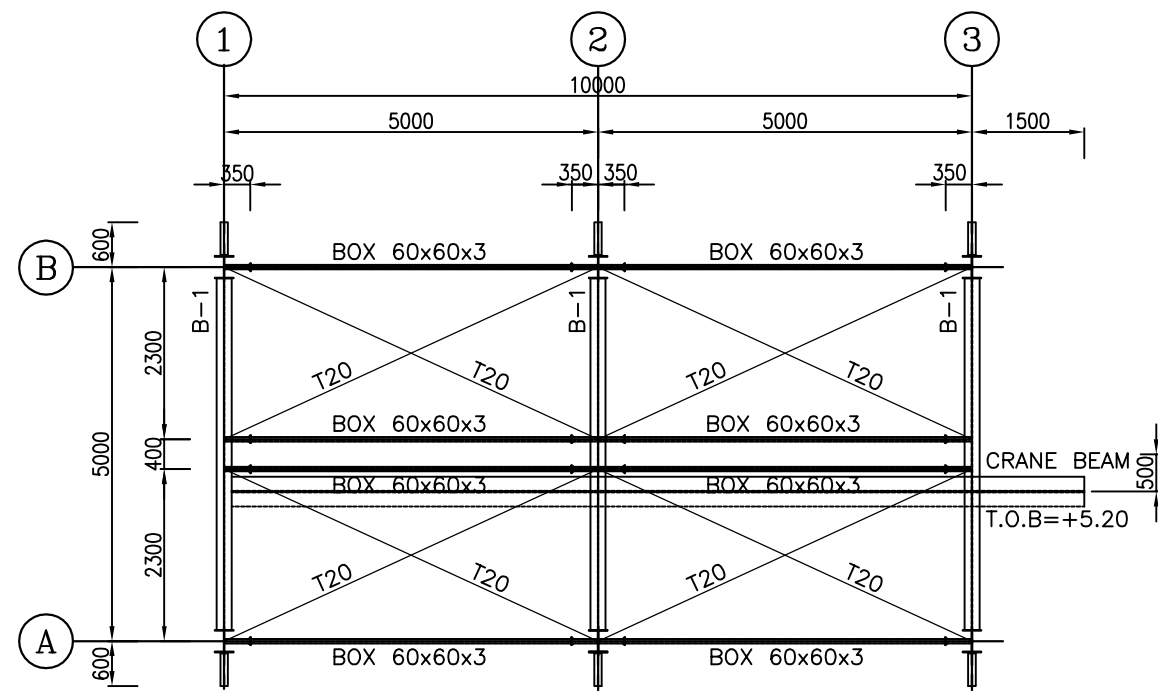
1:100 2 ROOF HORIZONTAL BRACING PLAN
