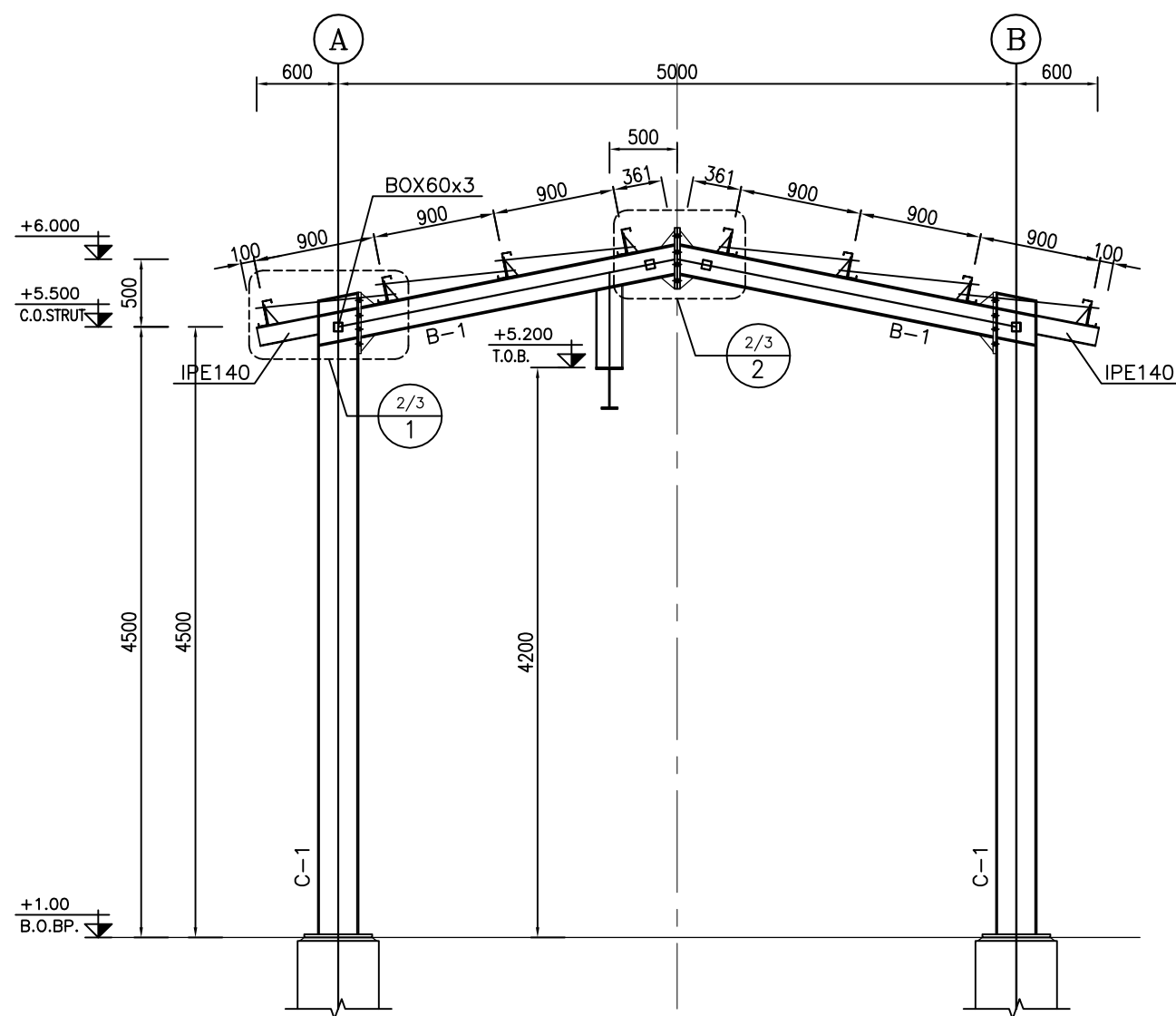
1:50 8 FRAMING ELEVATION ON AXIS 2
