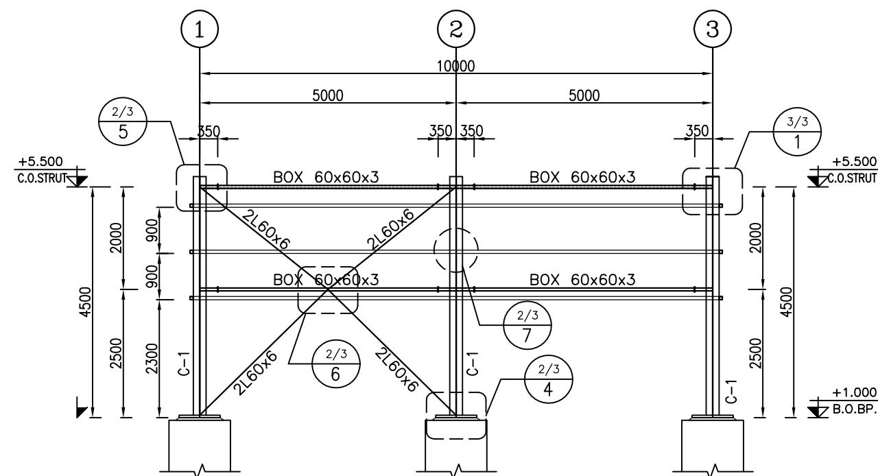
1:100 4 FRAMING ELEVATION ON AXES A&B
