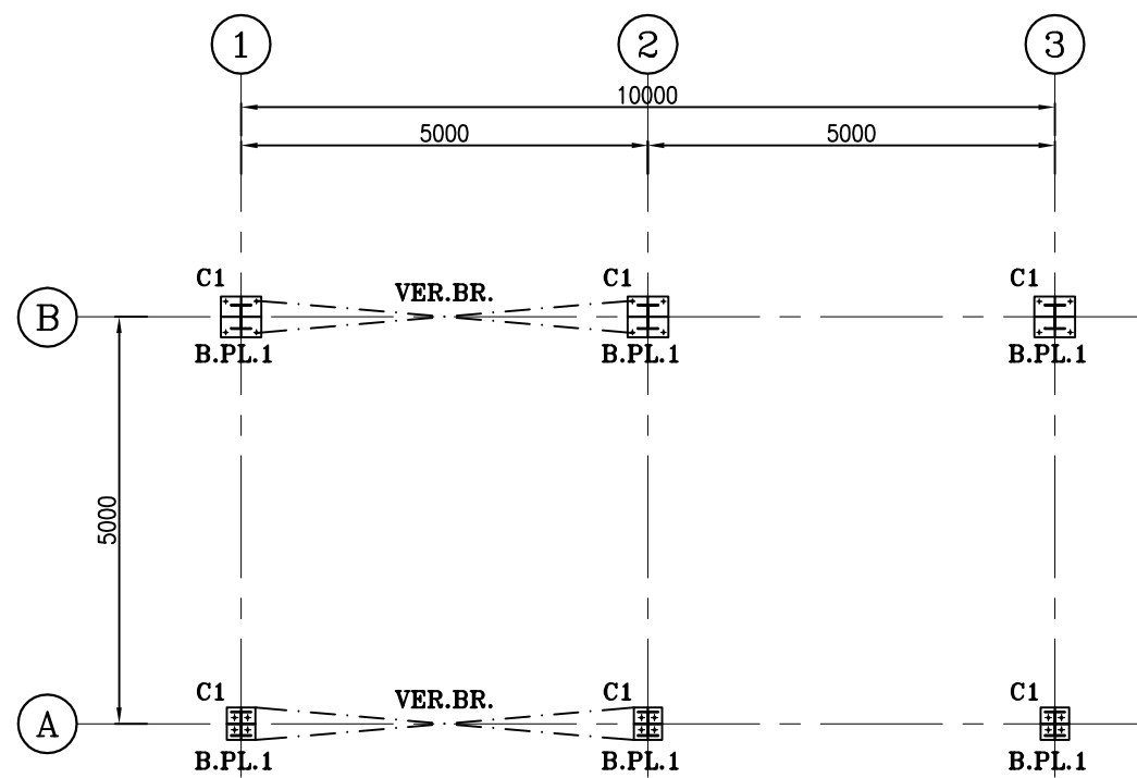
1:100 1 COLUMN & BASE PLATE LAYOUT PLAN
