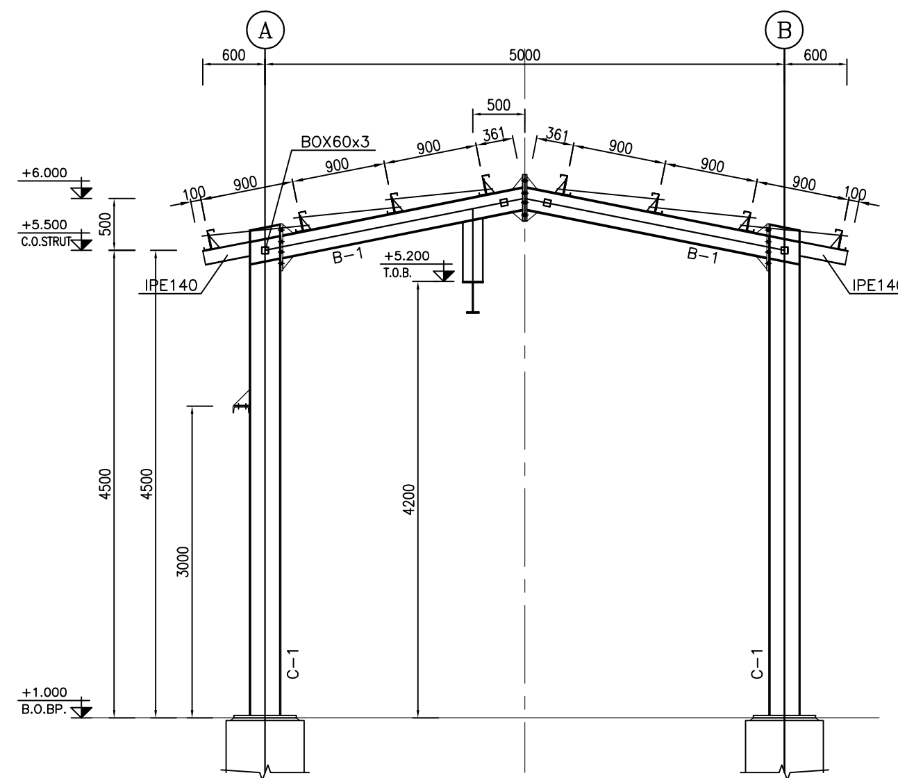
1:50 9 FRAMING ELEVATION ON AXES 3
