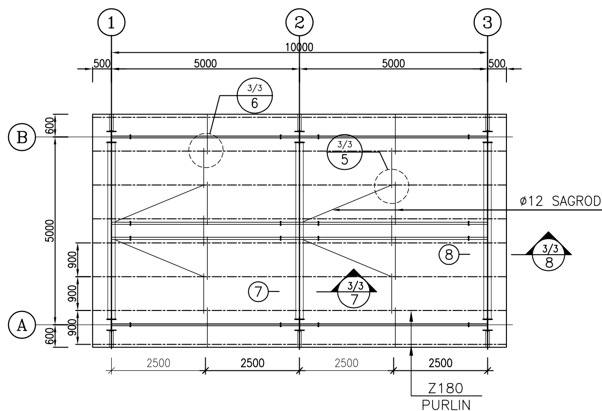
1:100 3 ROOF PURLIN PLAN
