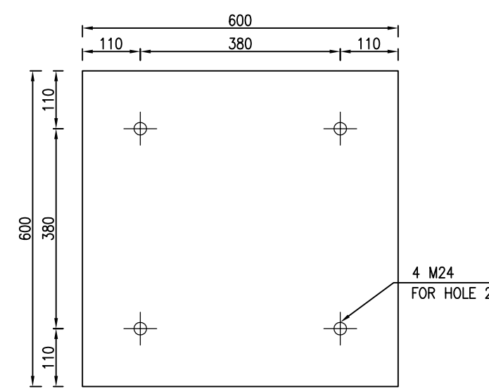
1:10 6 PEDESTAL 1 No.8
