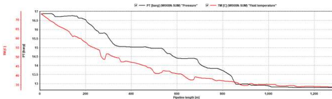
Curve 7-2.8: Temp/Press. Profile of 6" Asmari W008N Flow Line in summer (MIN-FLOW)
