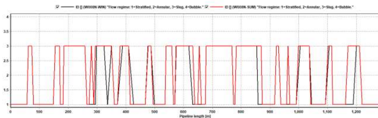
Curve 7-2.4: Flow Regime of W008N Asmari Flowline (MAX-FLOW)
