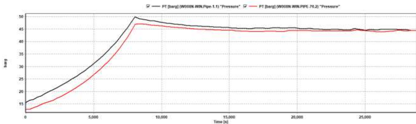
Figure 7-2.13: Surge Pressure for ASMARI Flow lines disposal wells (winter case)
