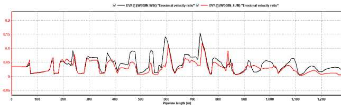
Curve 7-2.3: EVR of 6" Asmari Flowlines in Summer& Winter (MIN-FLOW)
