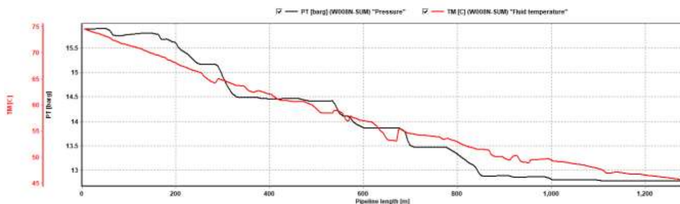
Curve 7-2.6: Temp/Press. Profile of 6" Asmari W008N Flow Line in summer (MAX-FLOW)
