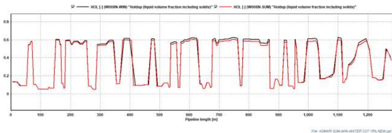
Curve 7-2.10: HOL. Profile of 6" Asmari W008N Flow Line in winter, summer (MAX-FLOW)
