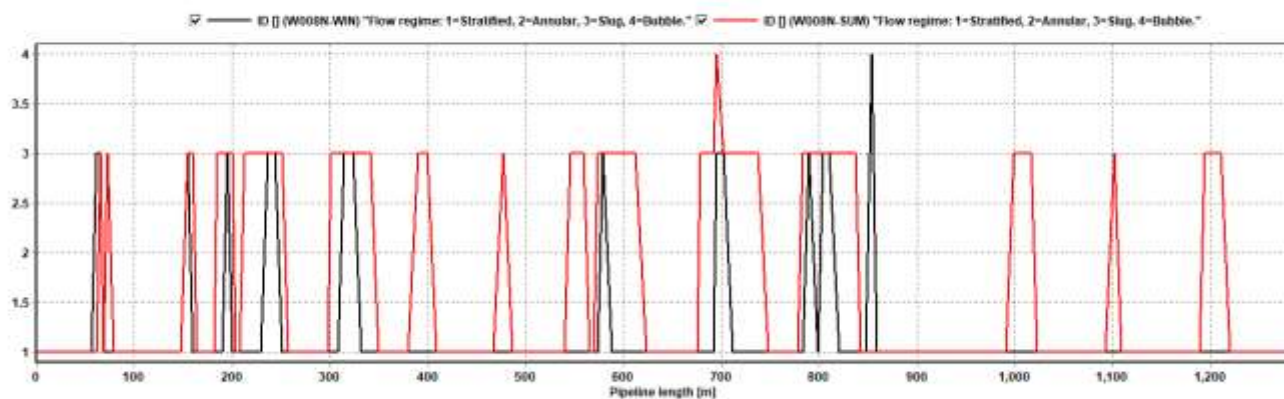
Curve 7-2.5: Flow Regime of W008N Asmari Flowline (MIN-FLOW)
