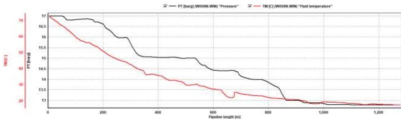
Curve 7-2.9: Temp/Press. Profile of 6" Asmari W008N Flow Line in winter (MIN-FLOW)
