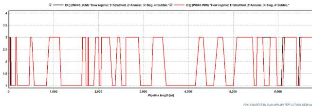
Curve 7-2.3: Flow Regime of W046 Bangestan Flowline (MAX-FLOW)
