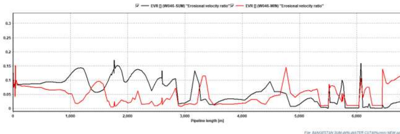
Curve 7-2.2: EVR of 6" Bangestan Flowlines in Summer& Winter (MIN-FLOW)
