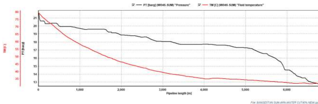
Curve 7-2.5: Temp/Press. Profile of 6" Bangestan W046S Flow Line in summer (MAX-FLOW)
