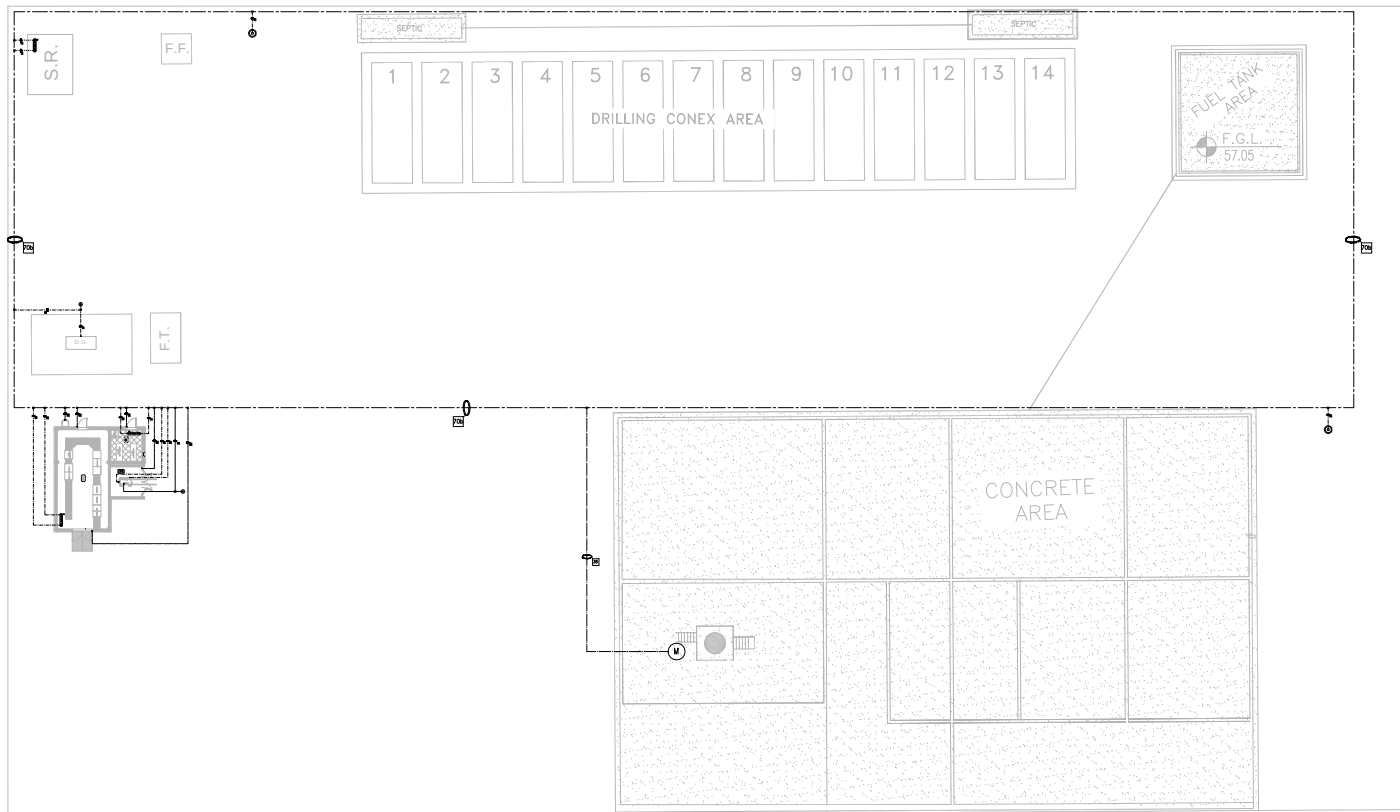
EARTHING LAYOUTS FOR WELLS NO. BK-12, BK-15, BK-14, W-007S & W-046S
