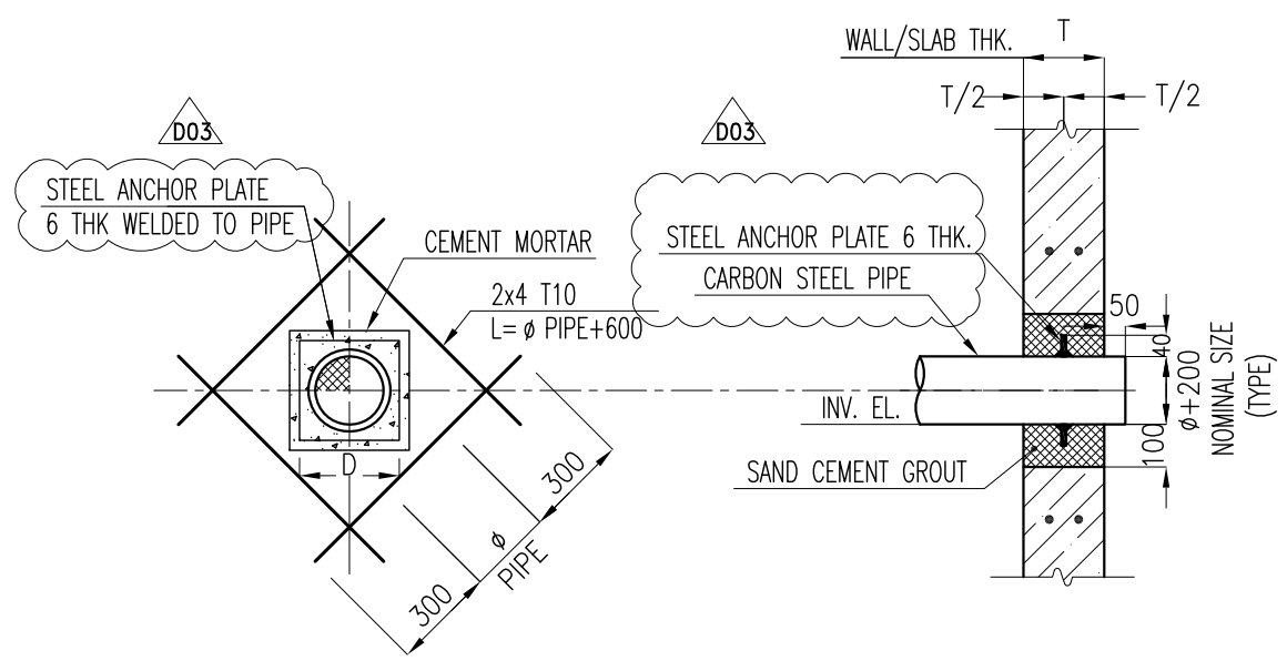
N.T.S 3 OPENNING REINFORCEMENT (TYPICAL FOR INLET/OUTLET PIPE)
