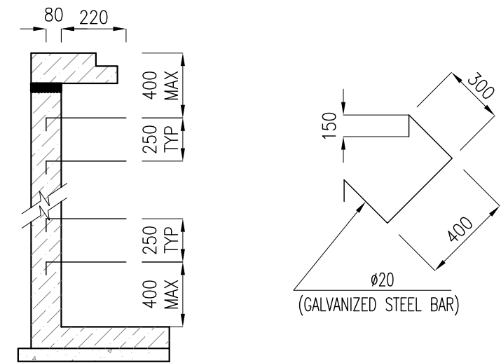
N.T.S 2 LADDER RUNGS DETAIL (ONLY FOR H ≥ 1050)
