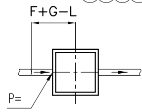
N.T.S 3 OPENNING REINFORCEMENT (TYPICAL FOR INLET/OUTLET PIPE)
