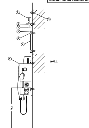
TELEPHONE SET (MTD. ON WALL)
