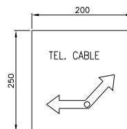
CABLE MARKER FOR BEND OF CABLE ROUTE
