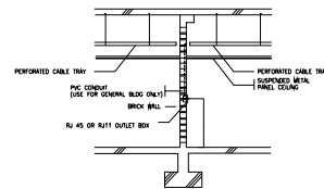
RJ 45/11 OUTLET FLUSH MOUNTED
