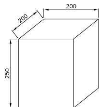
CONCRETE CABLE MARKER
