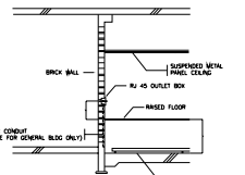
RJ 45 OUTLET SURFACE MOUNTED
