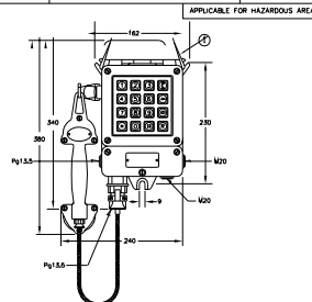
TELEPHONE OR HOTLINE HANDSET(EXPLOSION PROOF)
