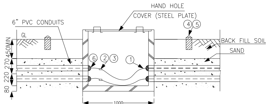
AROUND HAND HOLE
