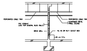
RJ 45 OUTLET FLUSH MOUNTED
