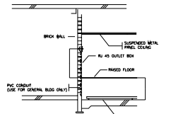
RJ 45/11 OUTLET SURFACE MOUNTED
