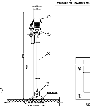
EX. TELEPHONE HANDSET (MTD ON POLE)
