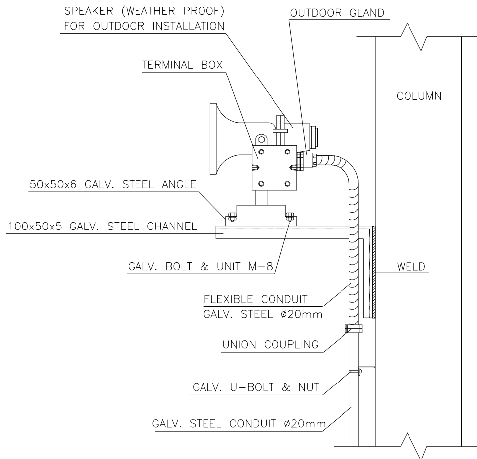
LOUD SPEAKER STRUCTURE MOUNTING OUTDOOR
