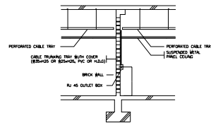
RJ 45 OUTLET SURFACE MOUNTED
