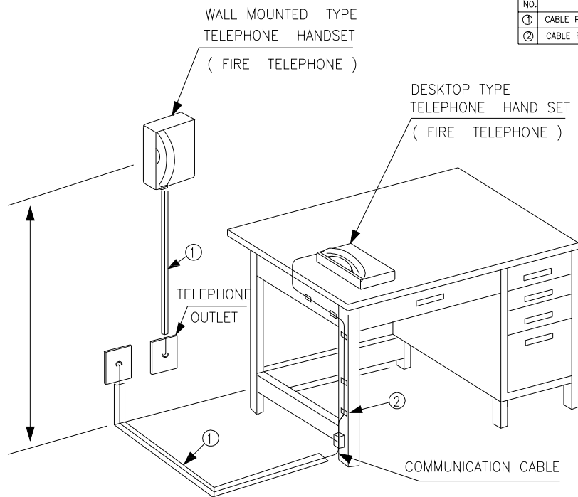
DESKTOP TELEPHONE OR HOTLINE TEL. (OFFICE)
