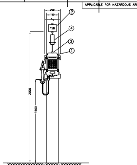
EX. TELEPHONE HANDSET (MTD ON STEEL STRUCTURE)
