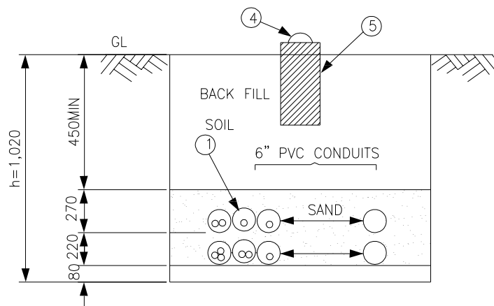
CABLE ROUTE (NON INDUSTRIAL AREA)
