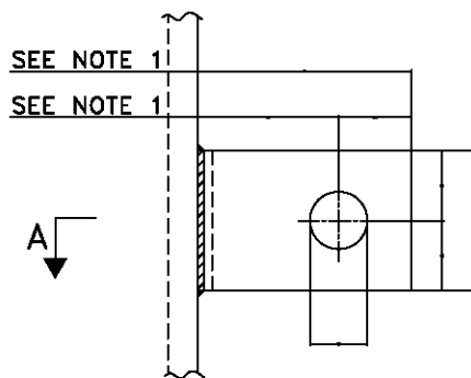
EARTHING TERMINAL DETAIL
