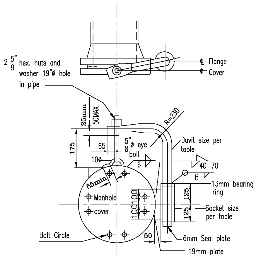
Manhole Cover Davit use for side entry
