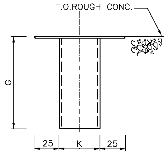
ELEVATION OF SLEEVE
