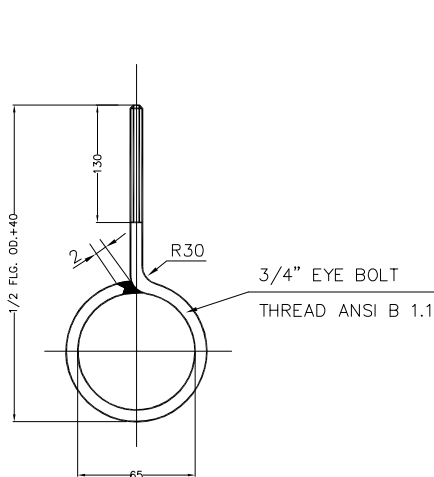
DETAIL 1 EYE BOLT
