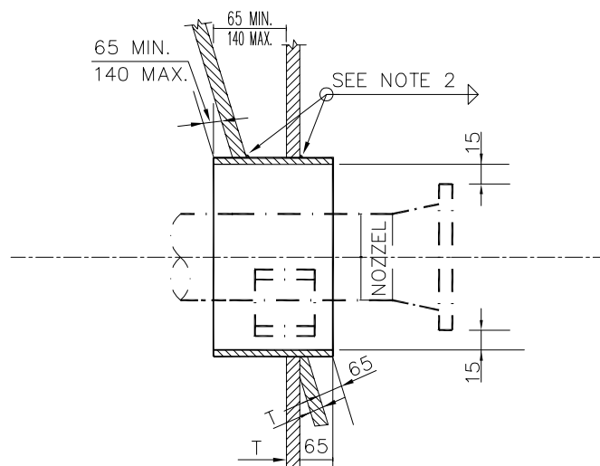
VIEW "A"
