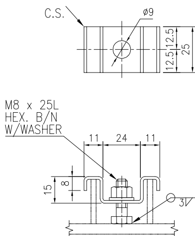
DETAIL OF SADDLE CLIP
