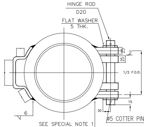
MANHOLE COVER HINGE USE FOR BOTTOM ENTRY
