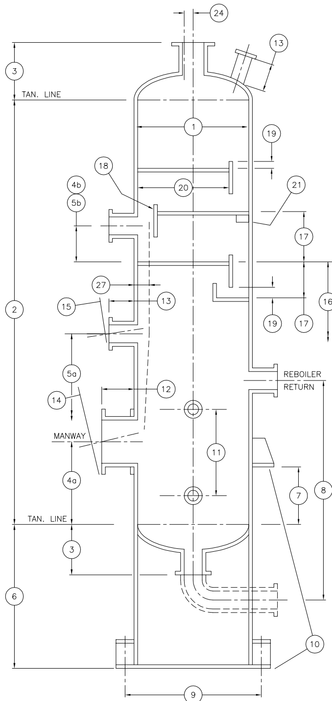
VERTICAL VESSEL
