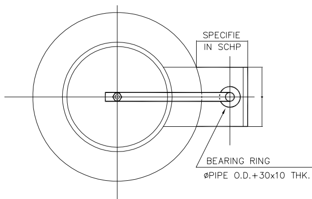
VERTICAL MANHOLE
