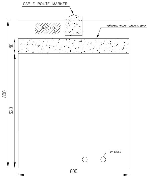
SECTION-01
