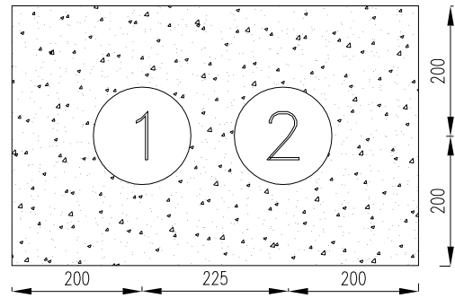
DUCT BANK-01
