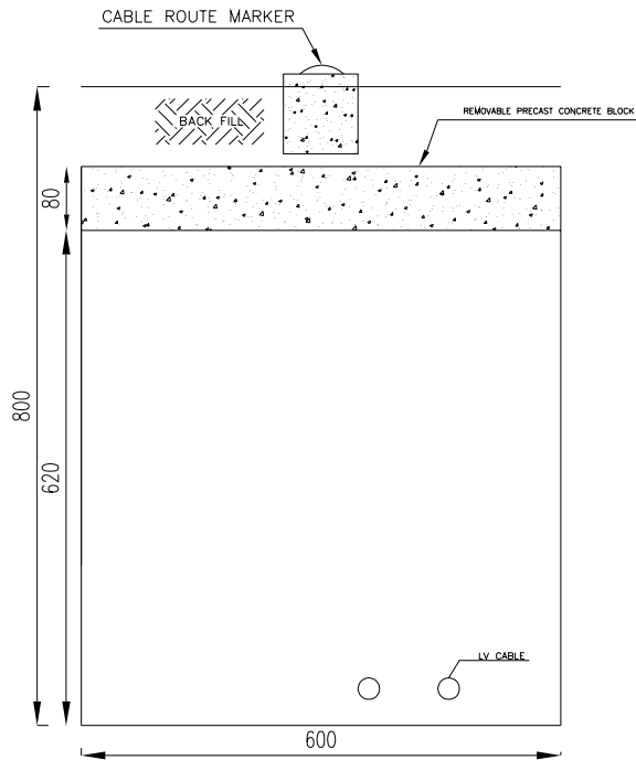
SECTION-02
