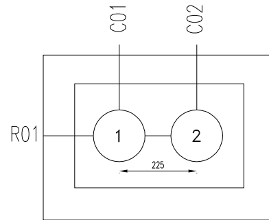
SECTION-10 SLEEVES
