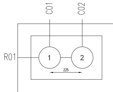
SECTION-15 SLEEVES
