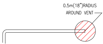
Figure 8- VENT SOURCE OF DIESEL STORAGE TANK
