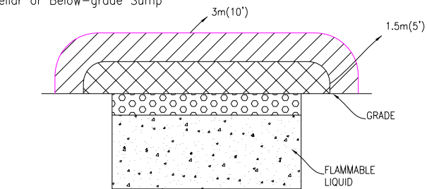
Figure 57-Open Sump in Non-enclosed, Adequately Ventilated Area
