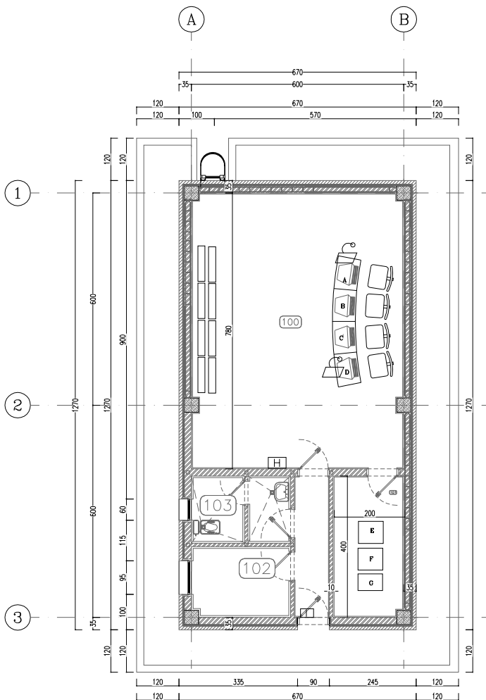
SC.1:50 1 DIMENSION PLAN
