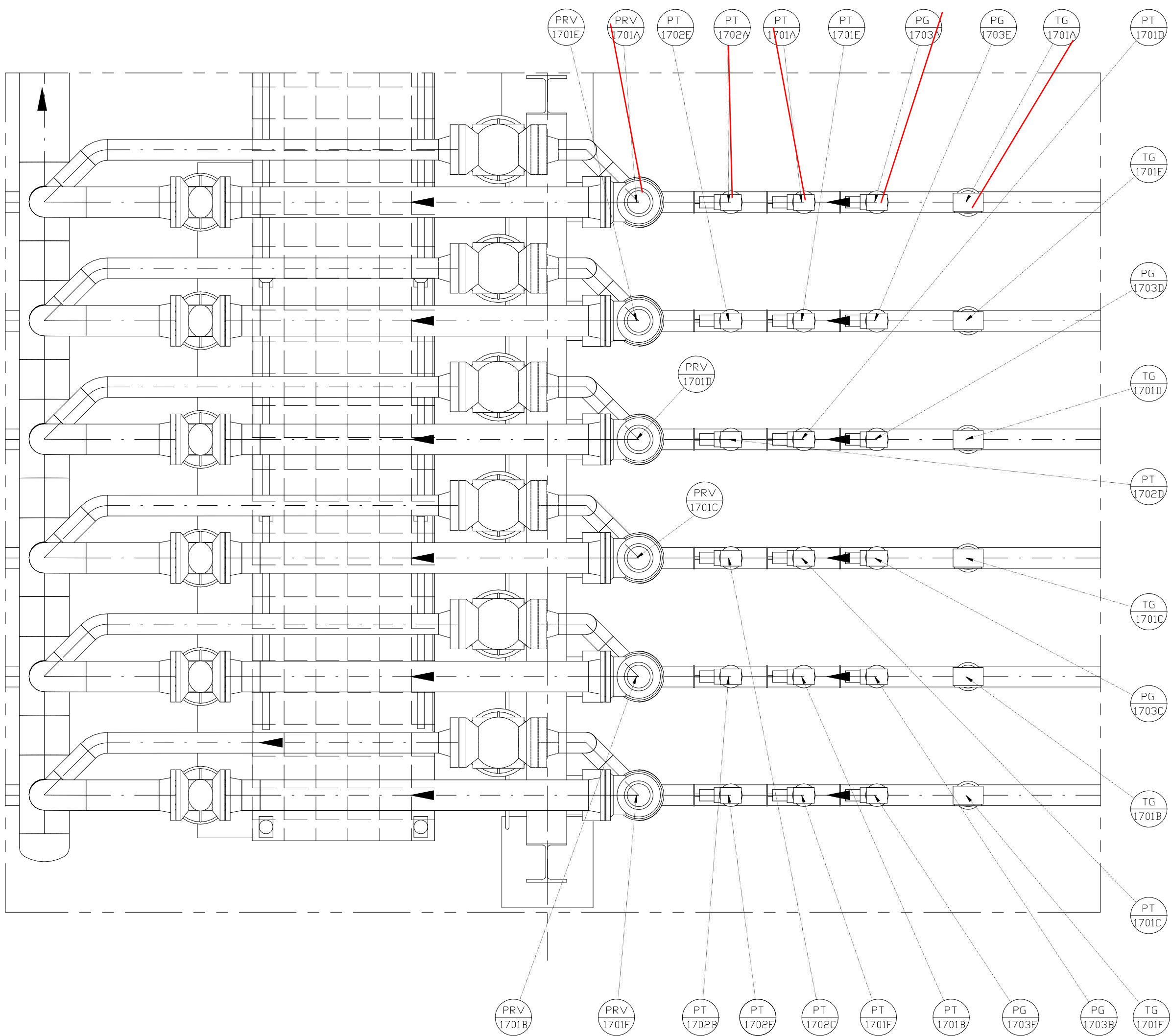
DETAIL A
