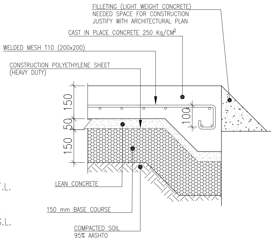
SECTION 7-7 Sc:1/25
