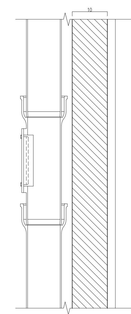
RAINWATER PIPE VALVE DETAIL Sc:1/25 DETAIL-01
