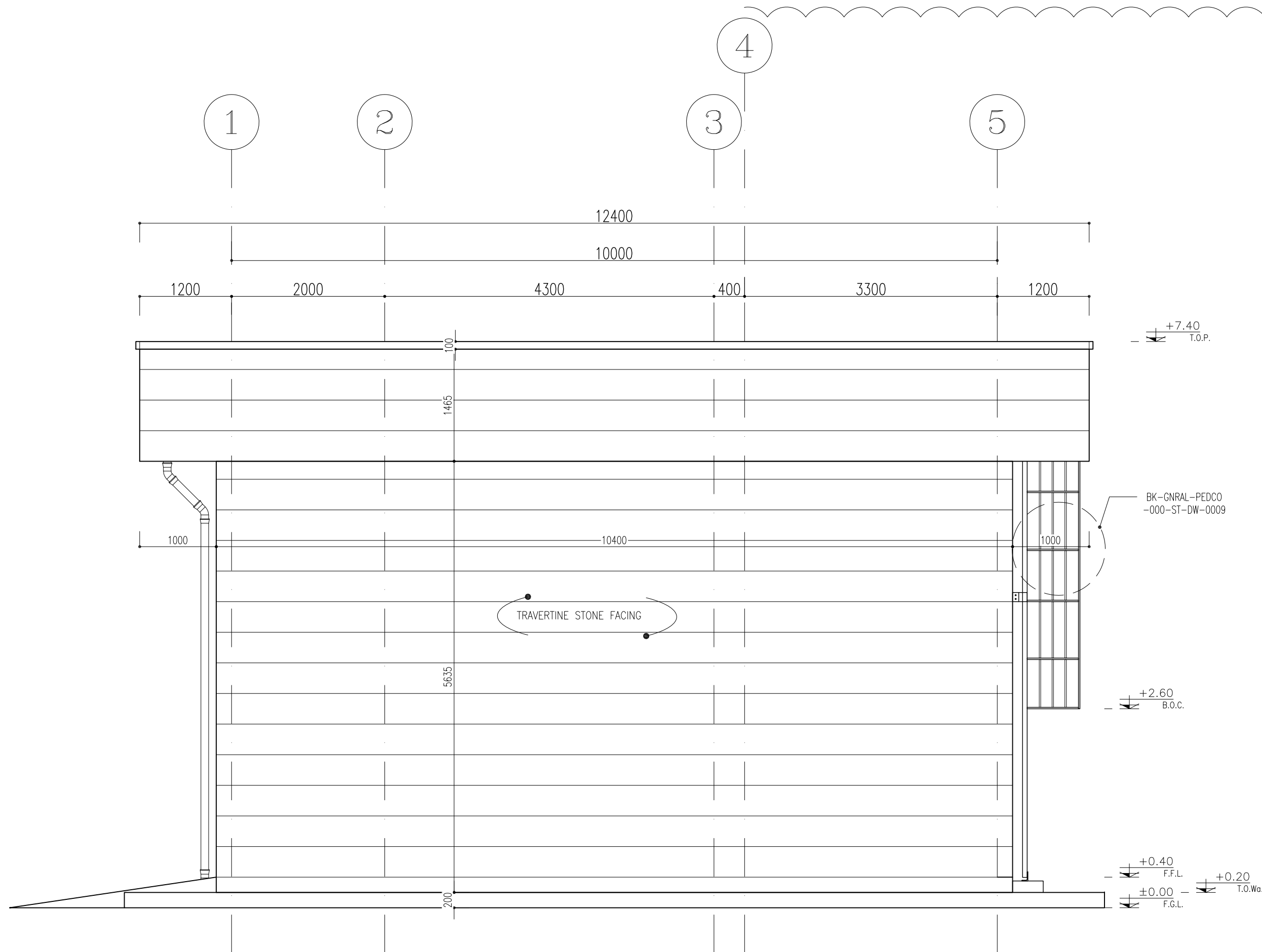
SC.1:50 2 01 OF 07 ELEVATION
