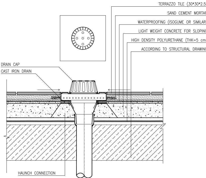
DRAIN DETAIL (ROOF) Sc:1/25 DETAIL-05
