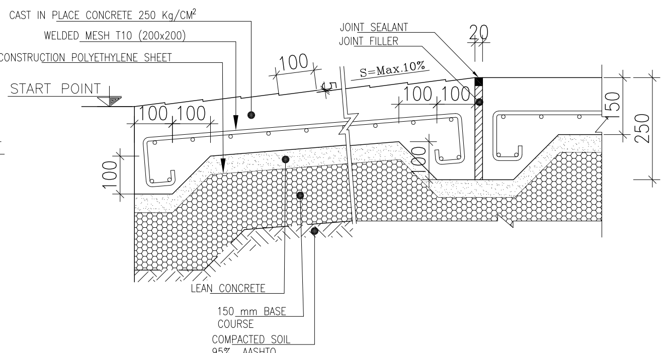
SECTION 8-8 Sc:1/25
