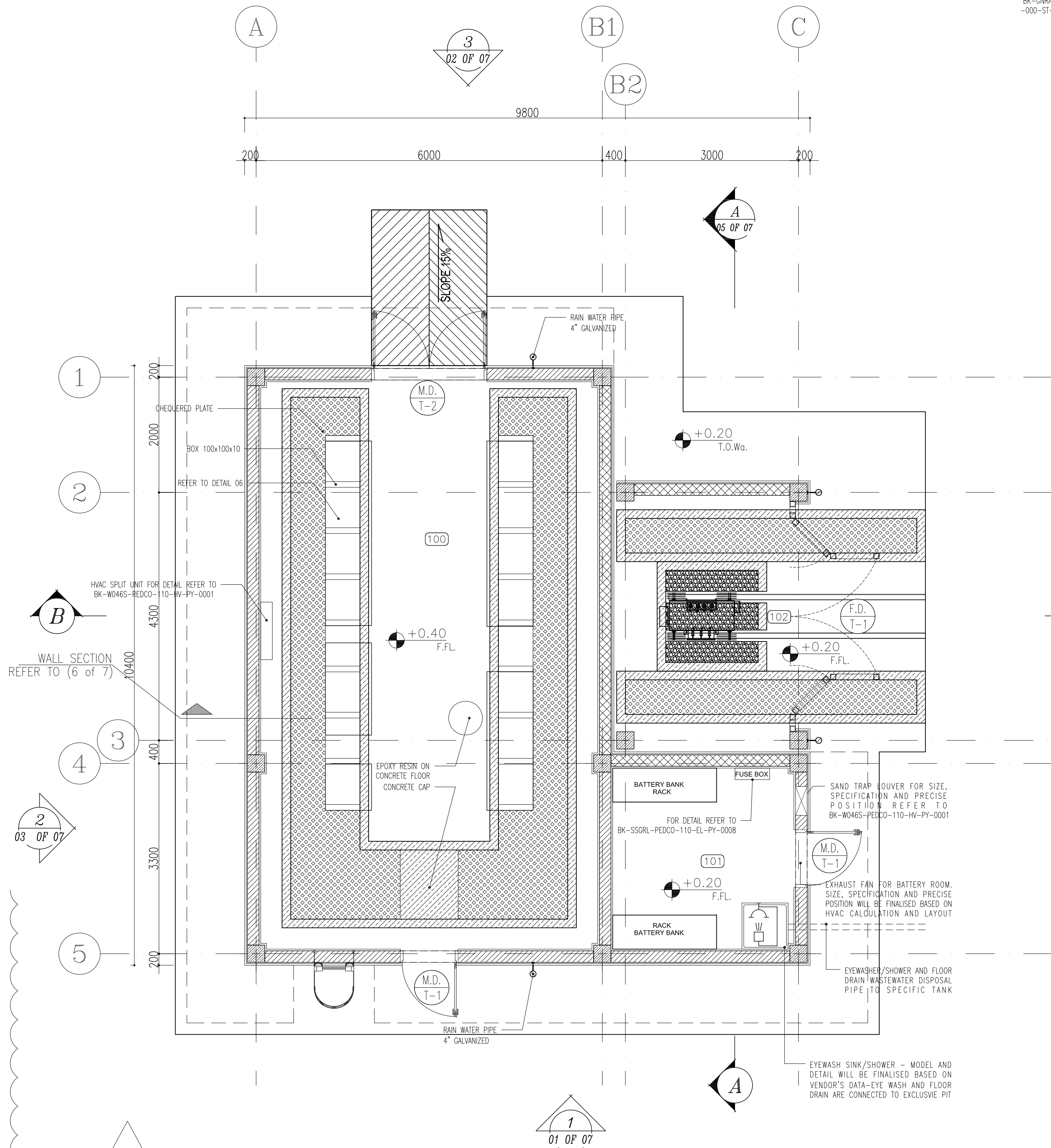
SC.1:50 1 PLAN
