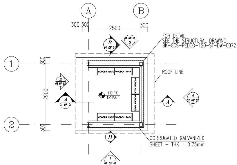
SC.1:50 1 GROUND FLOOR PLAN
