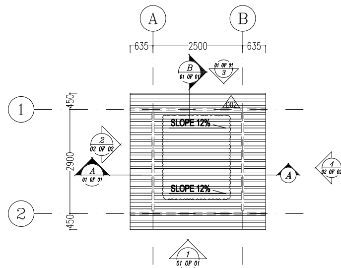
SC.1:50 2 ROOF PLAN
