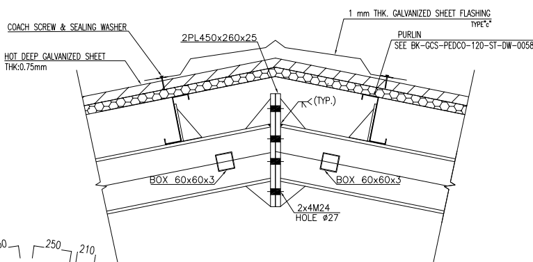
03 DETAIL 03 SC:1:10
