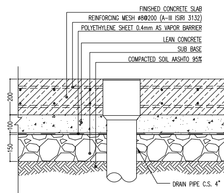
10 DETAIL 10 SC:1:10
