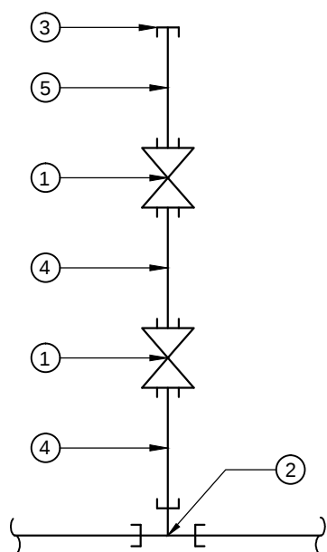
1 1/2" AND SMALLER (VENT)
