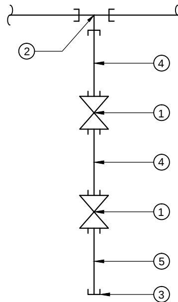
11/2" AND SMALLER (DRAIN)
