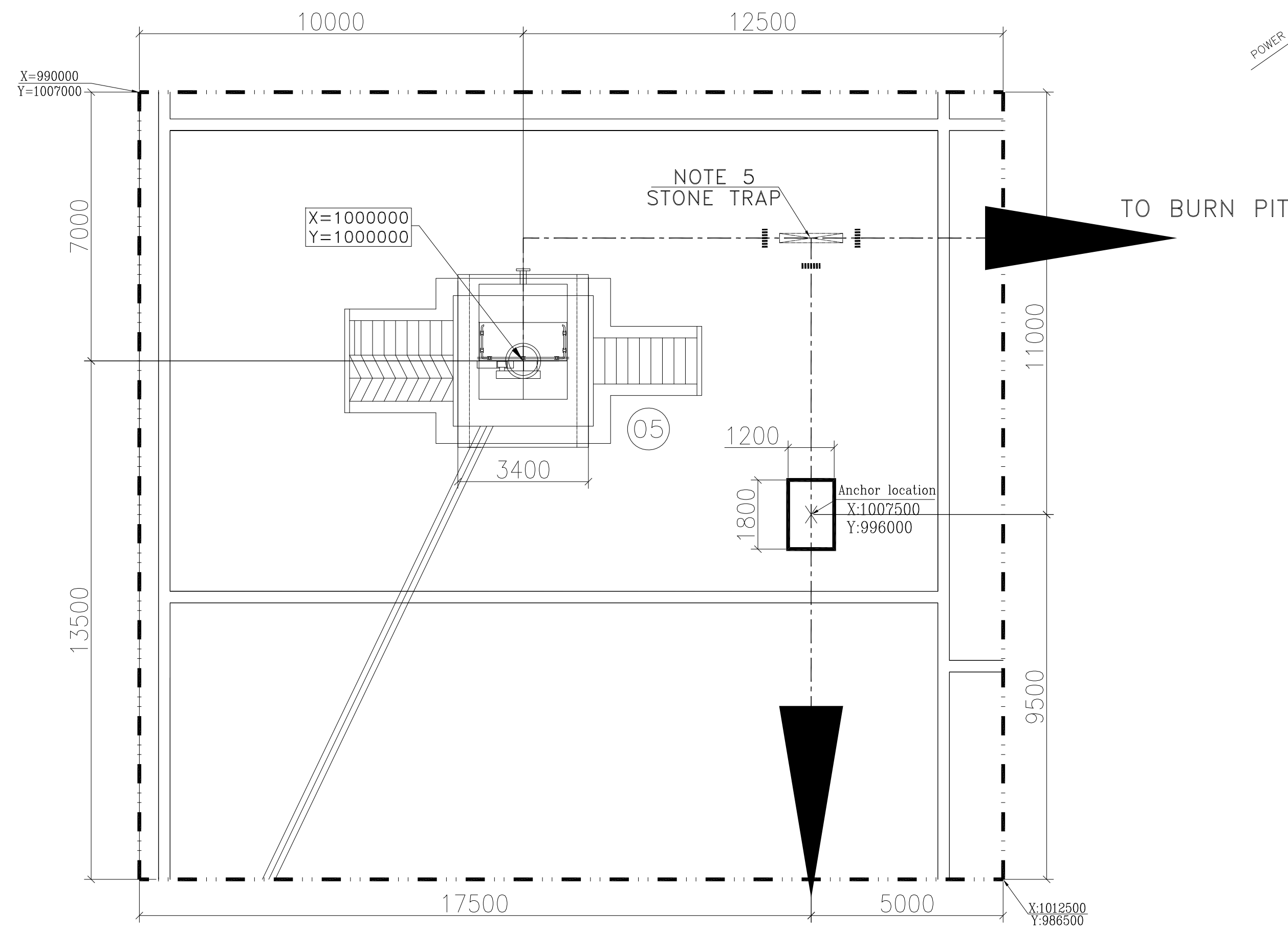
DETAIL A SC: 1/100
