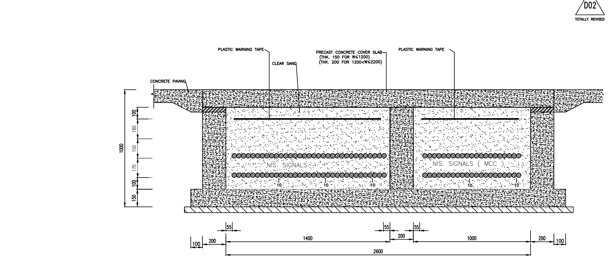
CONCRETE TRENCH SECTION A1B
