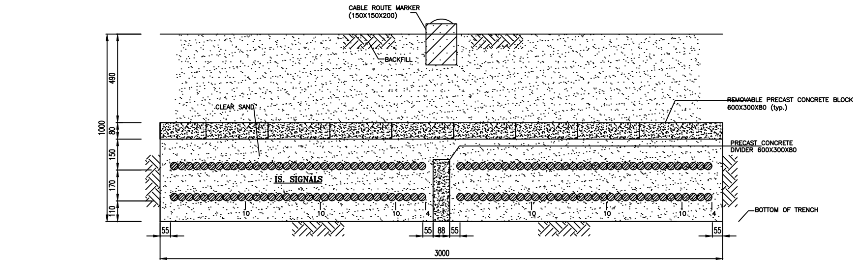
BURIED CABLE TRENCH
