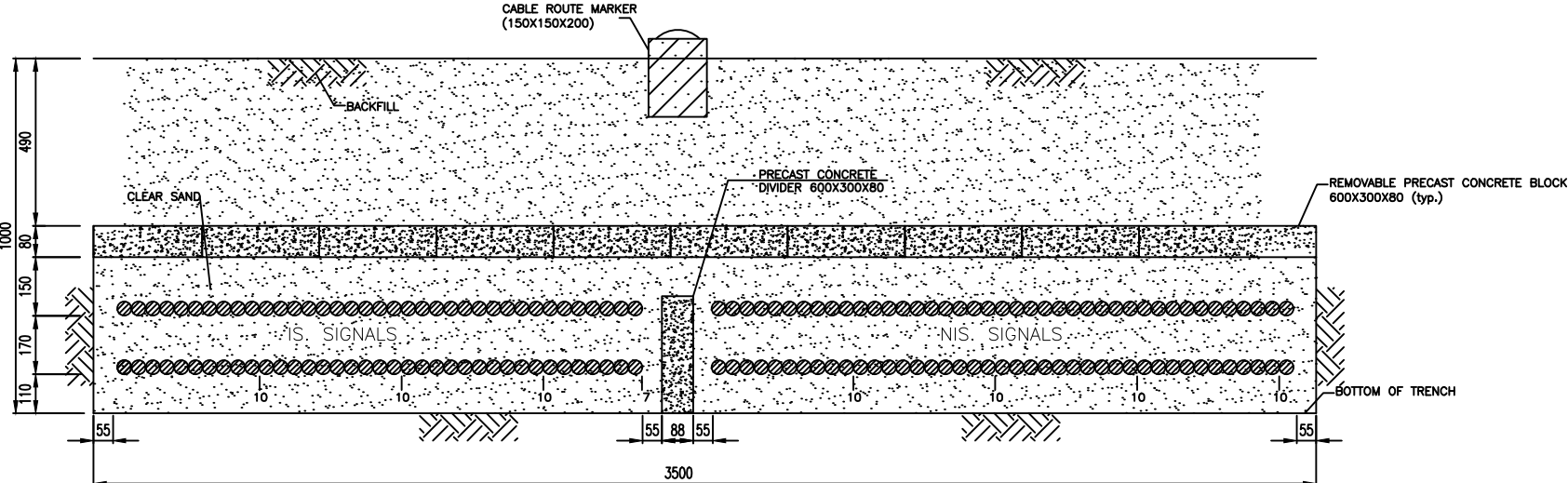
BURIED CABLE TRENCH SECTION A4
