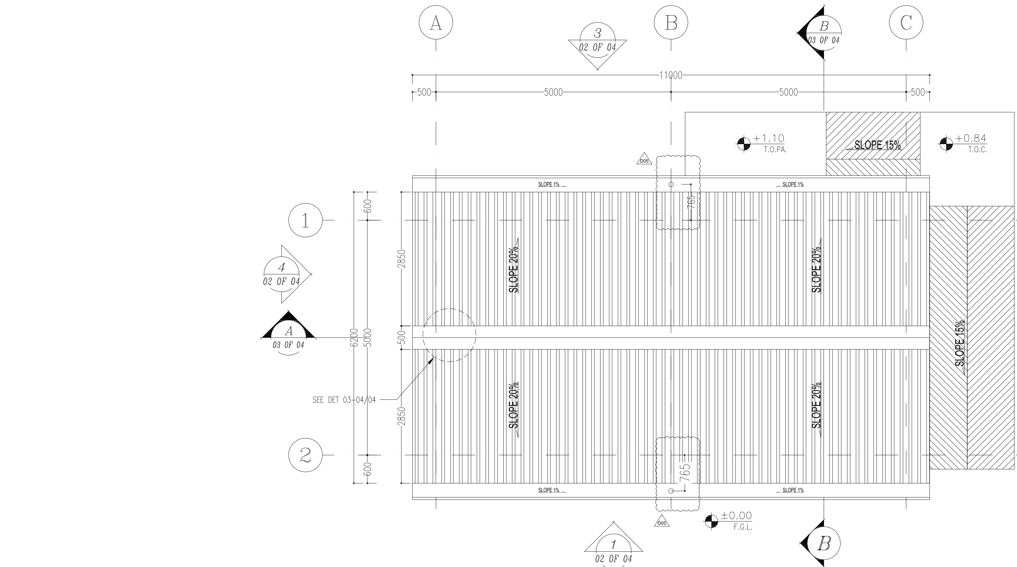
SC.1:50 2 ROOF PLAN
