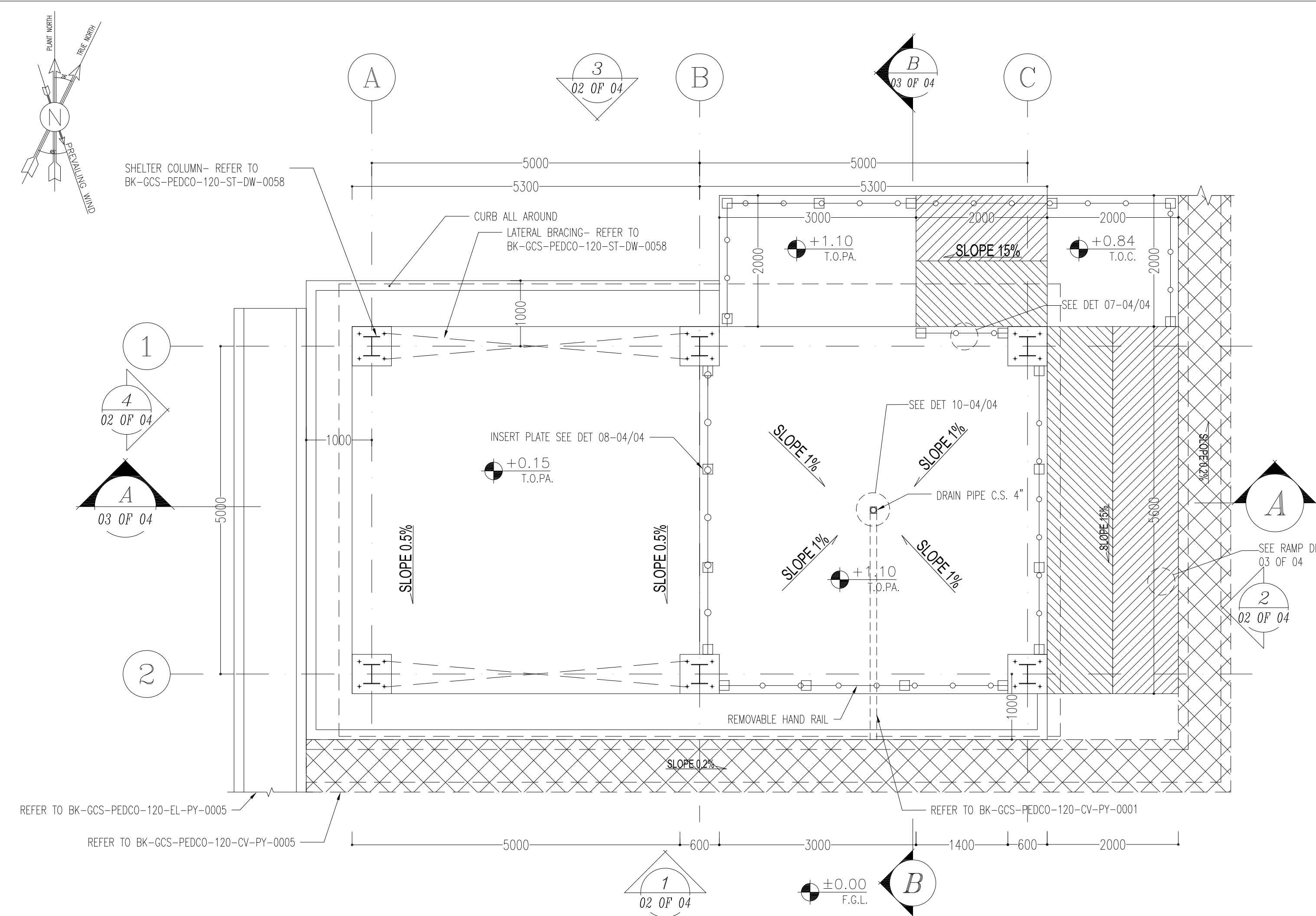
SC.1:50 1 FLOOR PLAN
