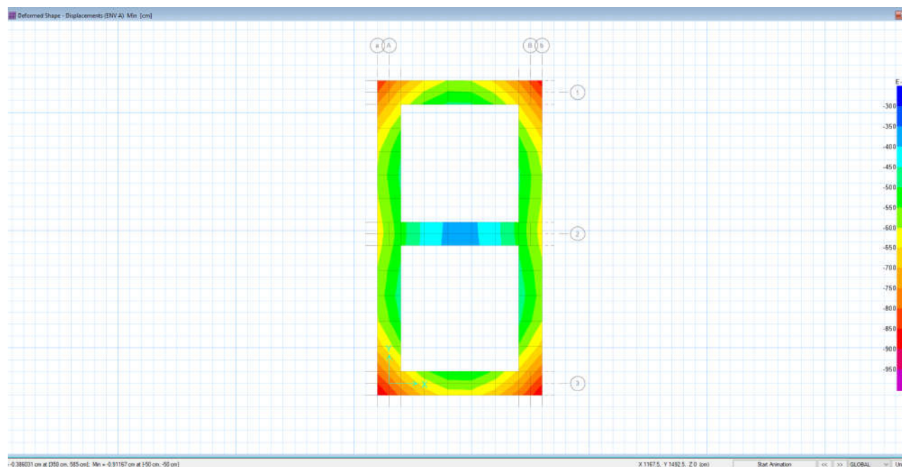
Figure 13: Foundation Settlement
