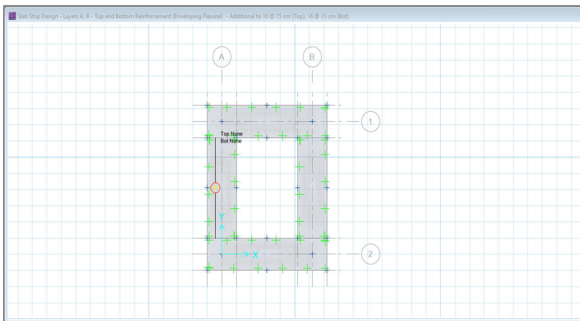
Figure 16: Reinforcement in X, Y Direction
