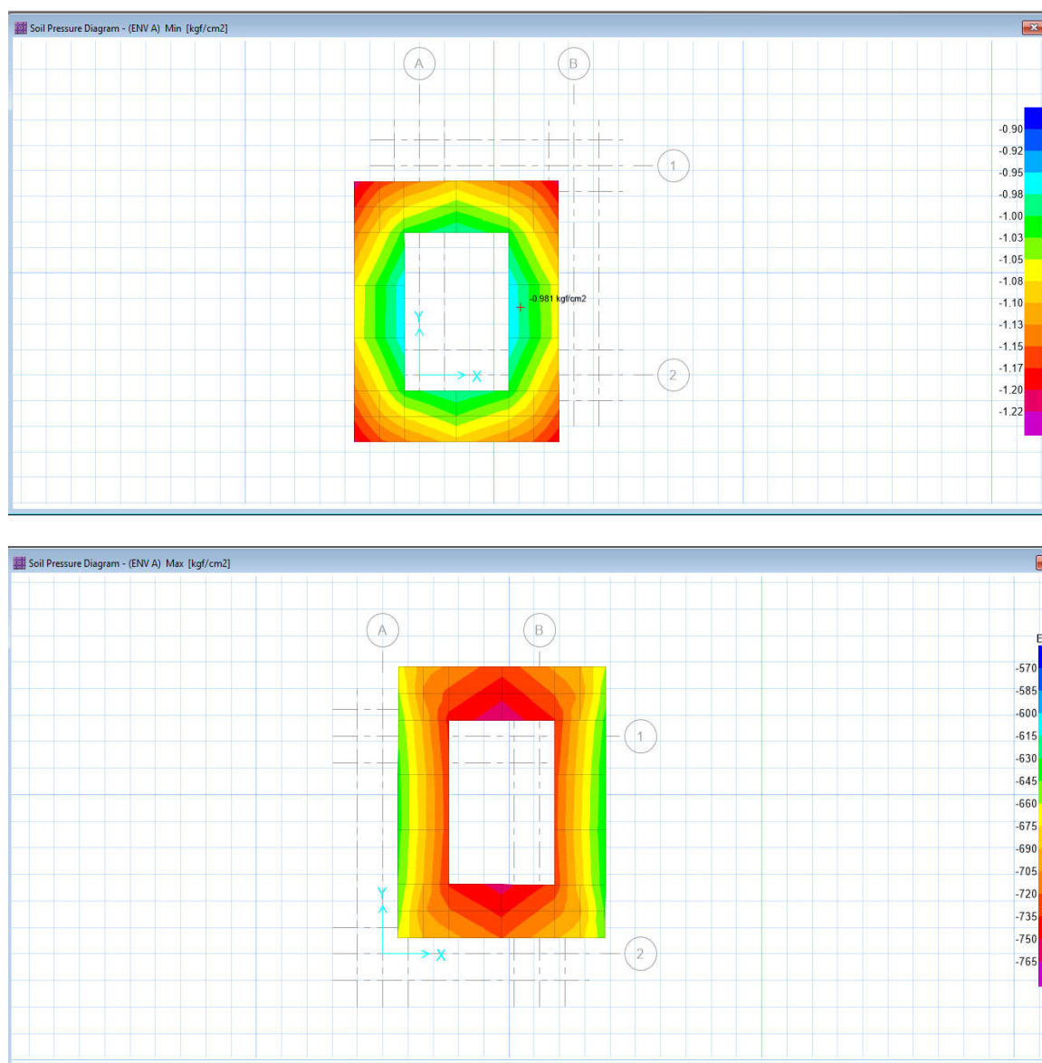
Figure 14: Soil Pressure under Foundation
