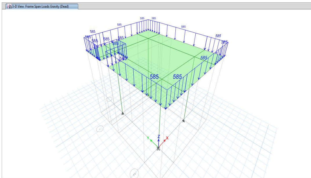
Figure 6: Parapet dead load
