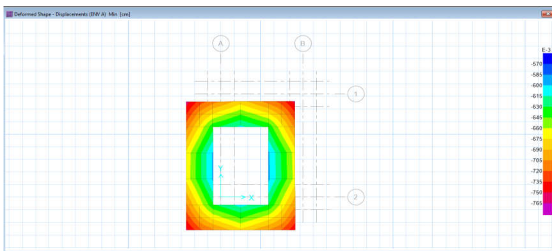
Figure 13: Foundation Settlement
