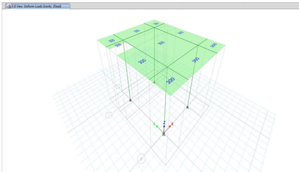
Figure 5: Dead load on roof
