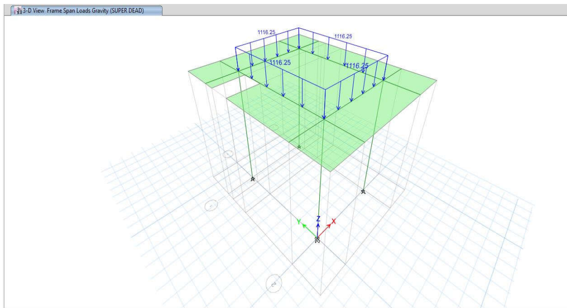
Figure 7: Dead load for wall
