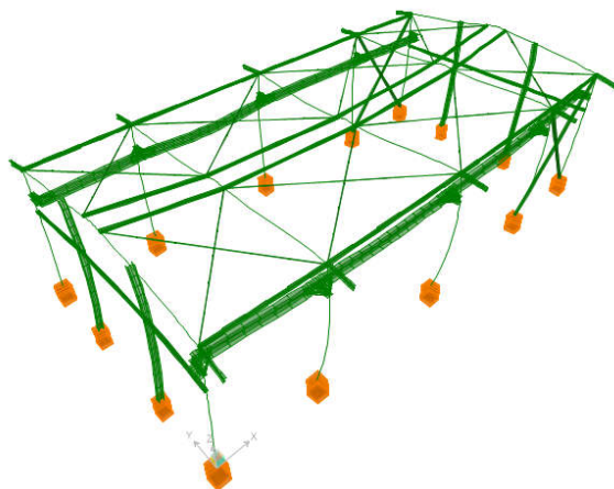
FIGURE 32: Deformed shape
