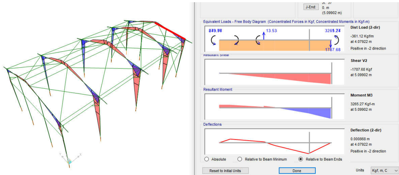
Figure 30: MOMENT 3-3 WY LOAD
