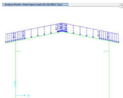
Figure 8-applied Snow load on middle axe 2,4(90.3 kg/m)
