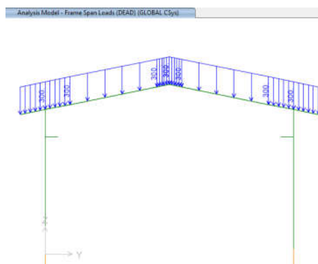
Figure 3-applied Dead load on frame 3(300 kg/m)
