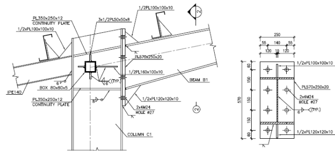
Figure 35: Connection Details
