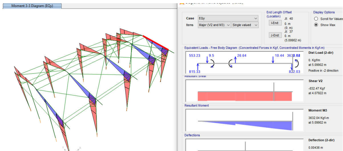
Figure 29: MOMENT 3-3 UNDER EY LOAD
