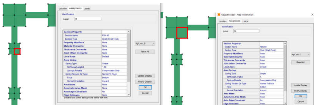
FIGURE 39-Assign Spring to Foundation(B=1m (ks=1.69kg/cm³)&B=2m(ks=1kg/cm³))
