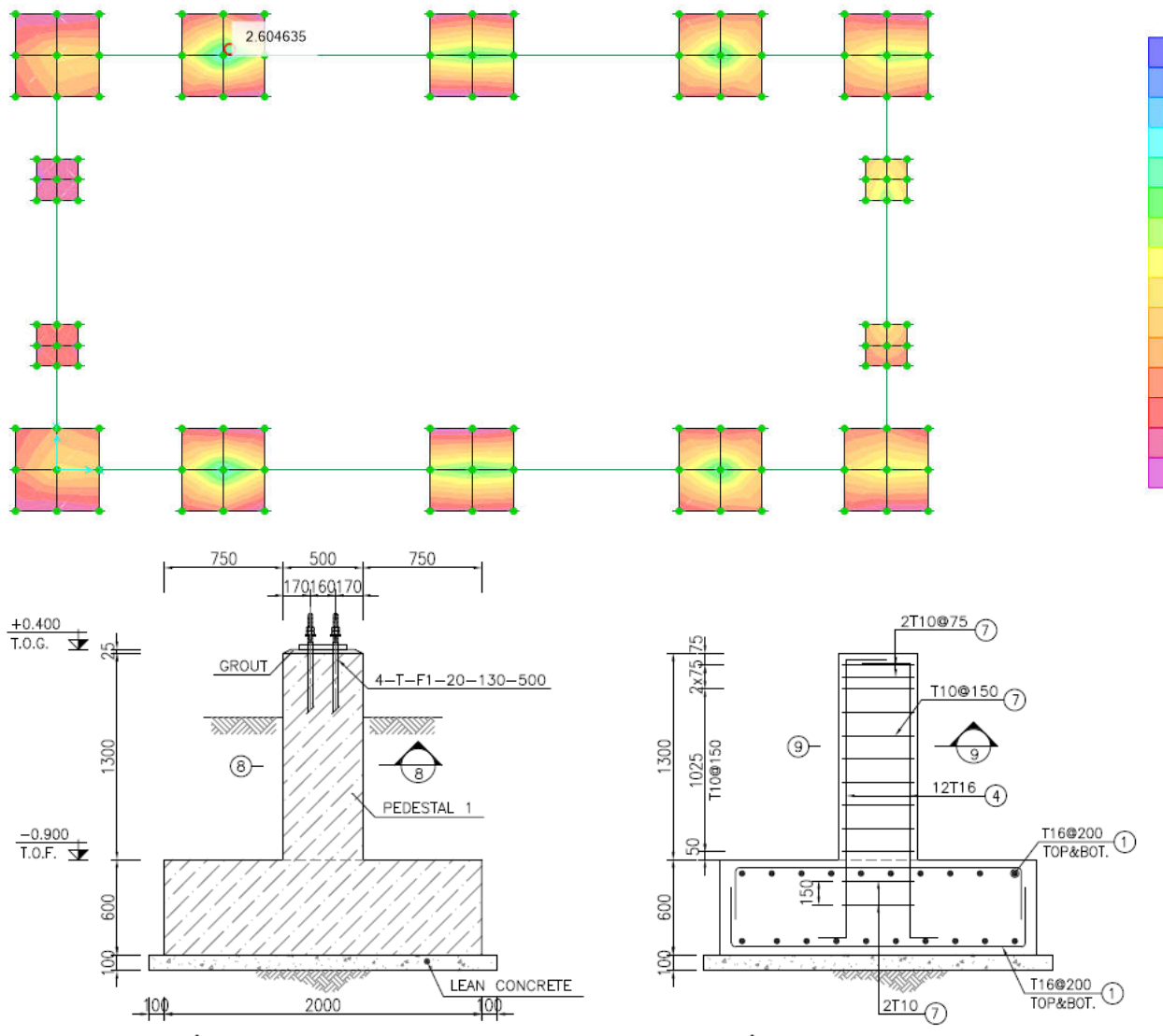
FIGURE 42-Reinforcement(Ø16@ 200)
