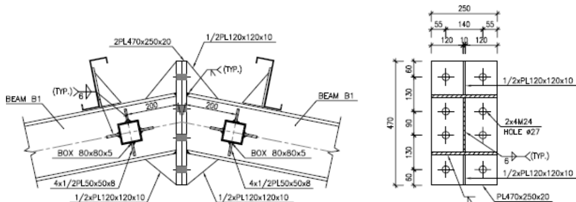
Figure 34: Connection Details
