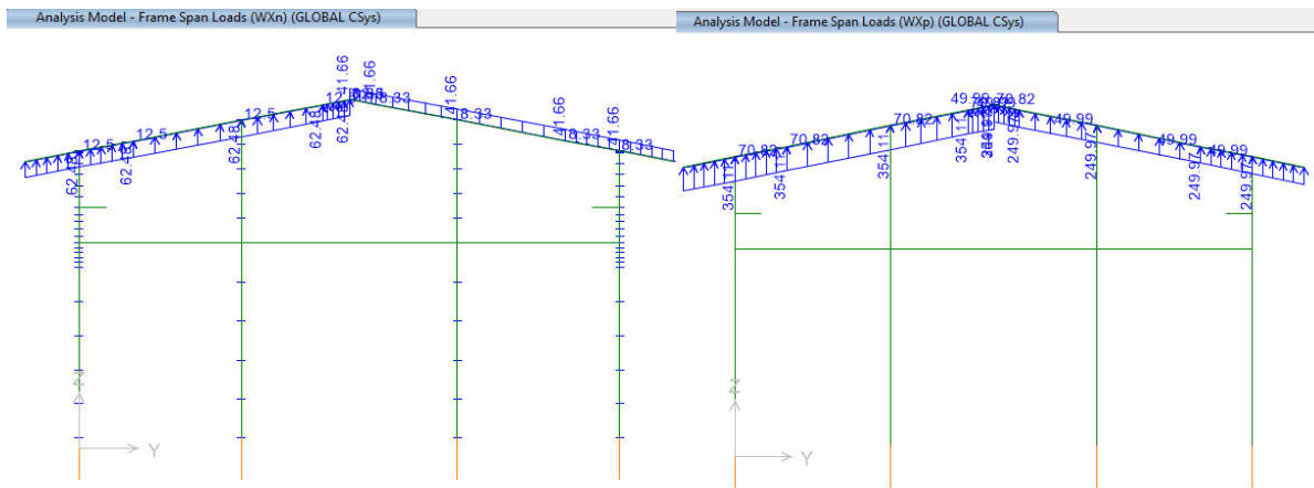
Figure 24-aplied Wind Load Applied frame A(Wxn:kg/m) Figure 25-aplied Wind Load Appliedframe A(Wxp:kg/m)
