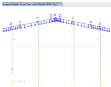
Figure 7-applied Snow load on ended axe(1&5) (36.12 kg/m)
