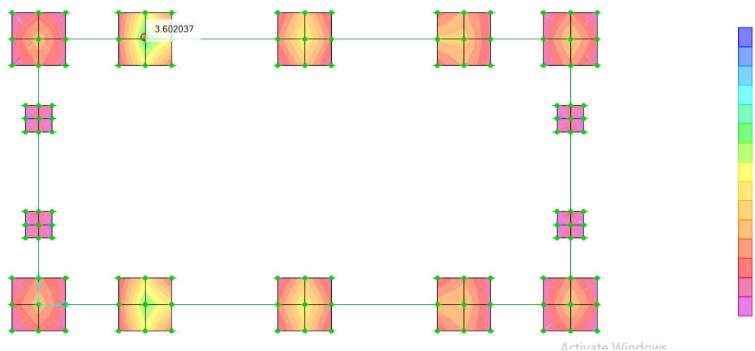
FIGURE 41-M22 & M11 result
