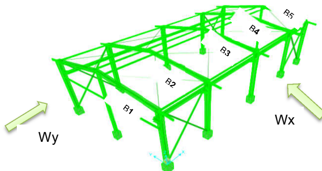
Figure 23-Wind Load Direction
