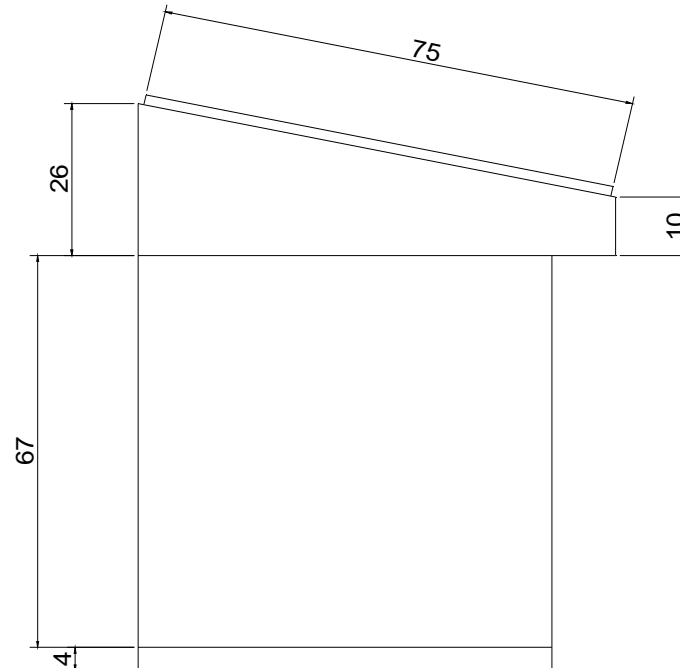
SIDE VIEW OF PANEL (TO BE FINALIZED BY VENDOR) ESD CONSOLE AND F&G CONSOLE HAVE SAME SEDIGN
