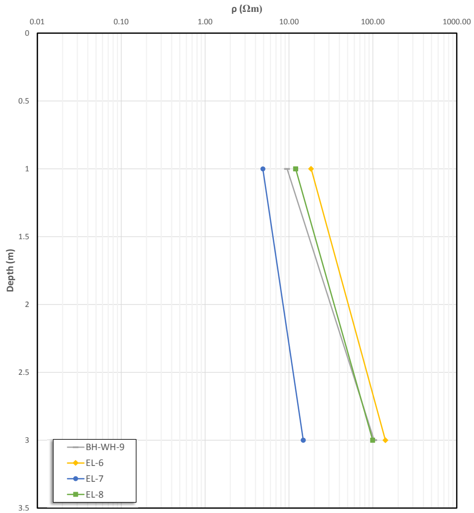
Variation of Apparant Electrical Resistivity in BK-12
