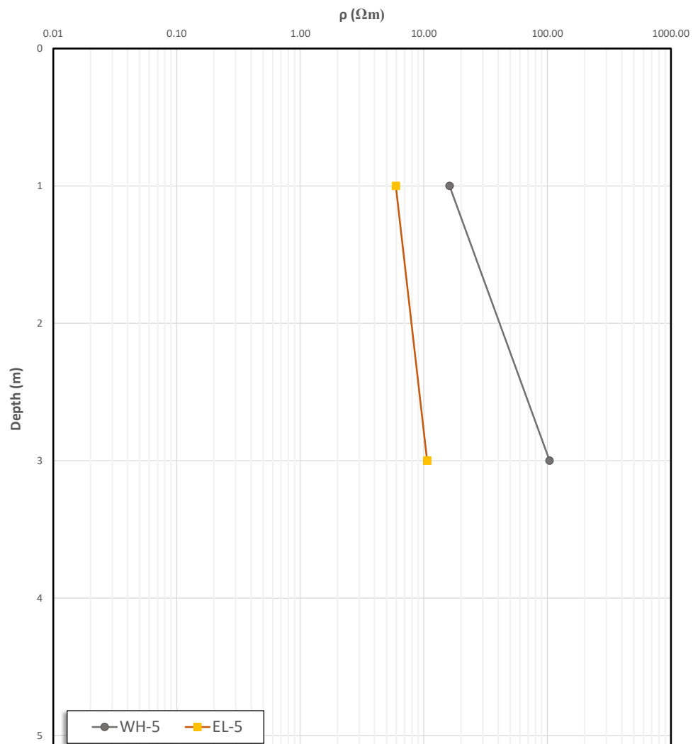
Variation of Apparant Electrical Resistivity in W-007S
