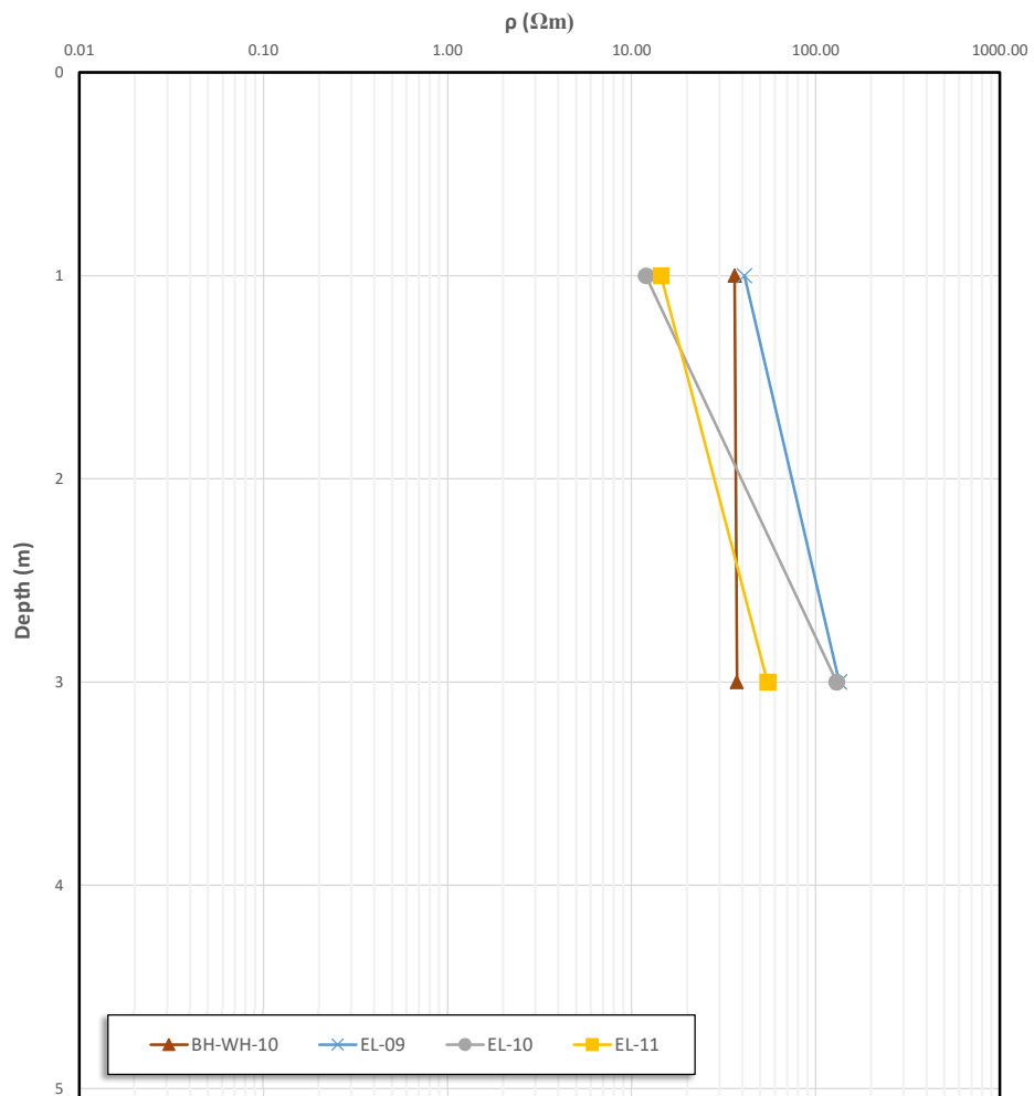
Variation of Apparant Electrical Resistivity in BK-14
