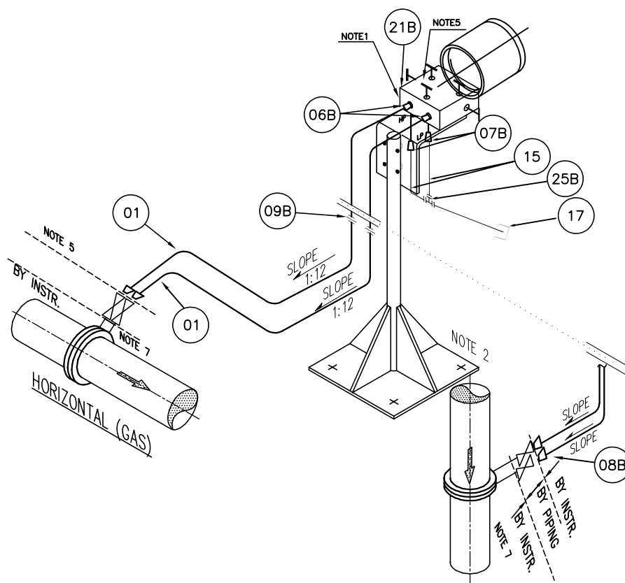
(DETAIL OF MANIFOLD ITEM 21)
