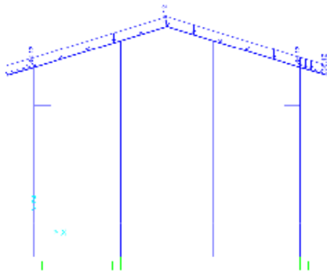
Figure 5-Applied Snow load on ended axes 1&4 (kg/m)
