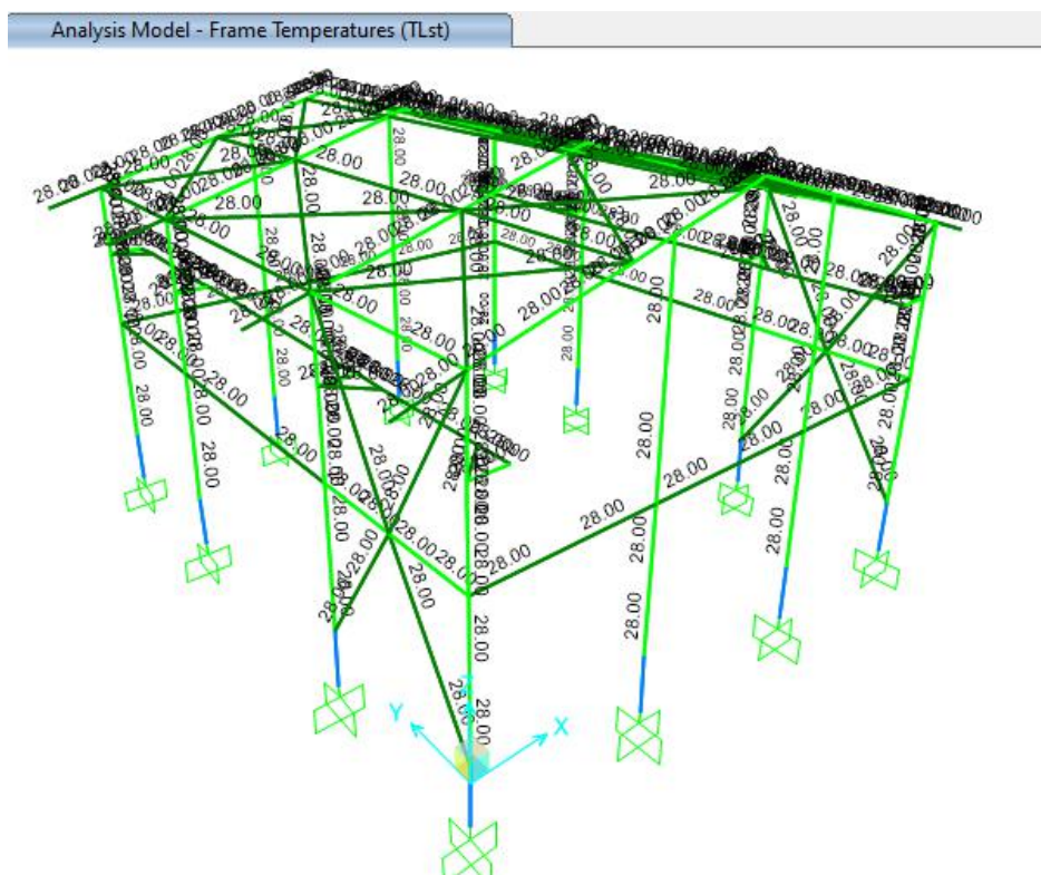
Figure 16-Applied Thermal Load (TLst) on Structure
