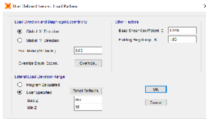
Fig 7- X Direction Seismic Load
