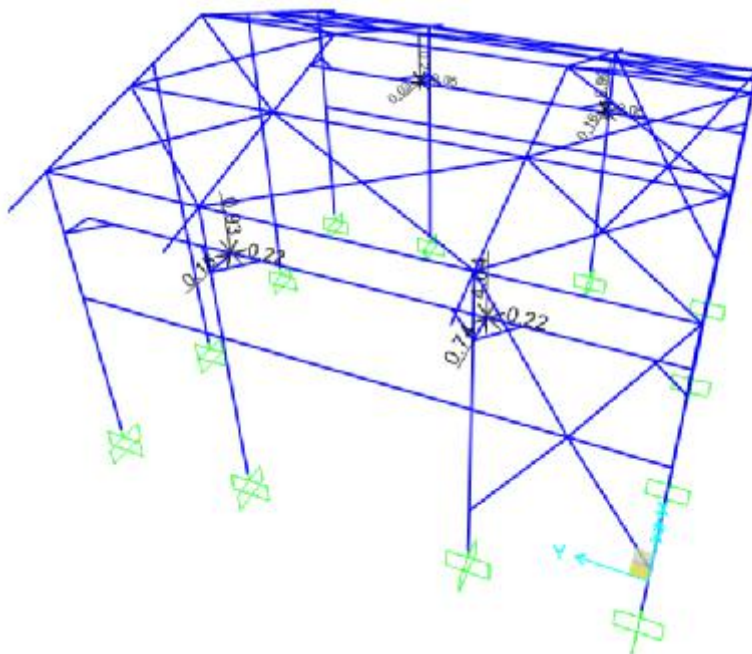
Figure 9-Applied Crane Operating load (CRO1) on Structure (ton)
