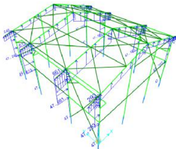
Figure 12-Applied Wind load (WLX1) on Structure (kg/m)
