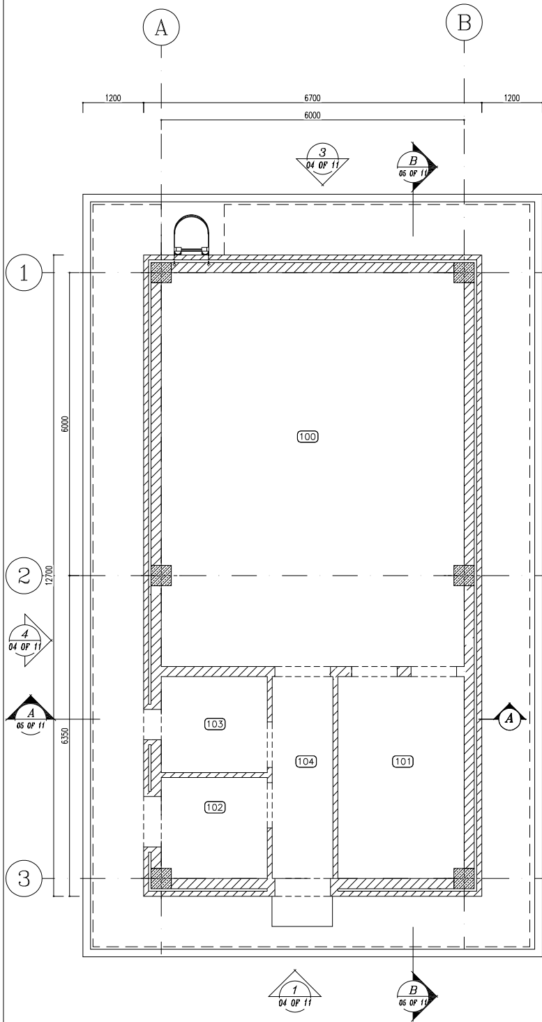
SC.1:50 4 LINTEL PLAN
