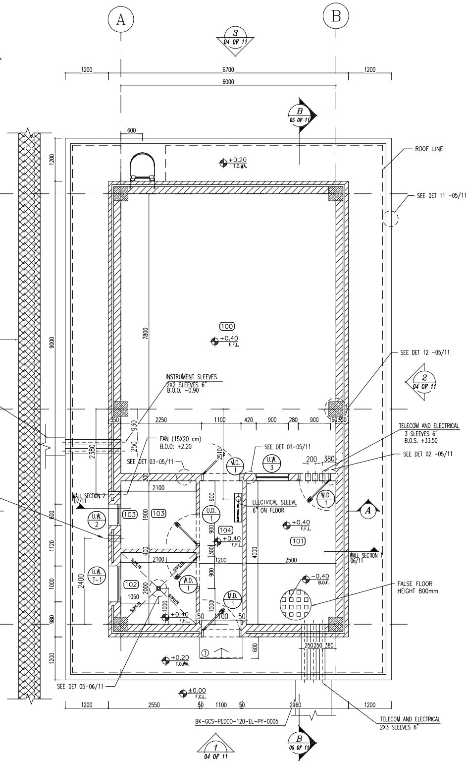
SC.1:50 1 DIMENSION PLAN
