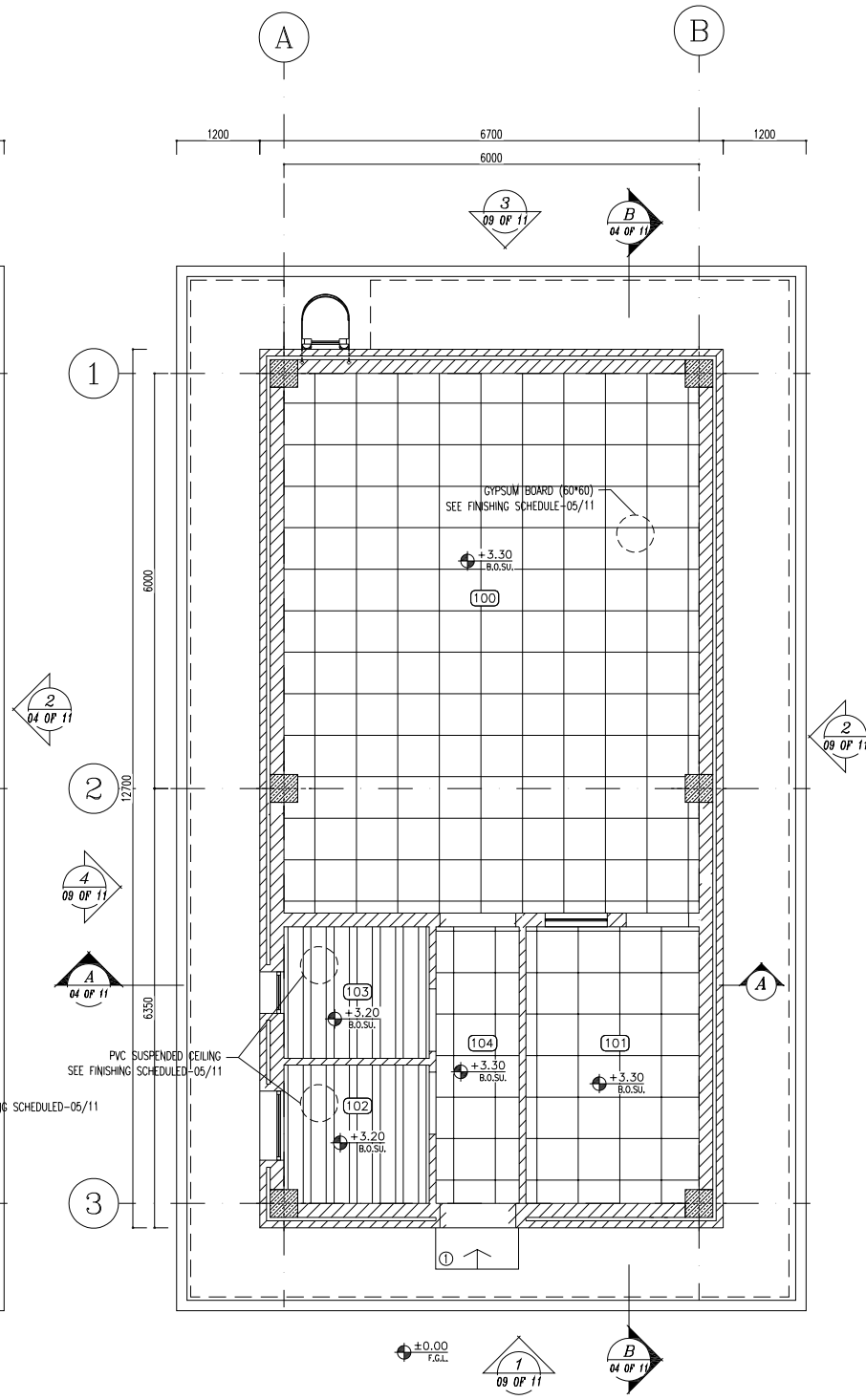
SC.1:50 4 SUSPENDED CEILING PLAN
