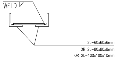
TYP. SECTION 1-1 Sc: 1:5
