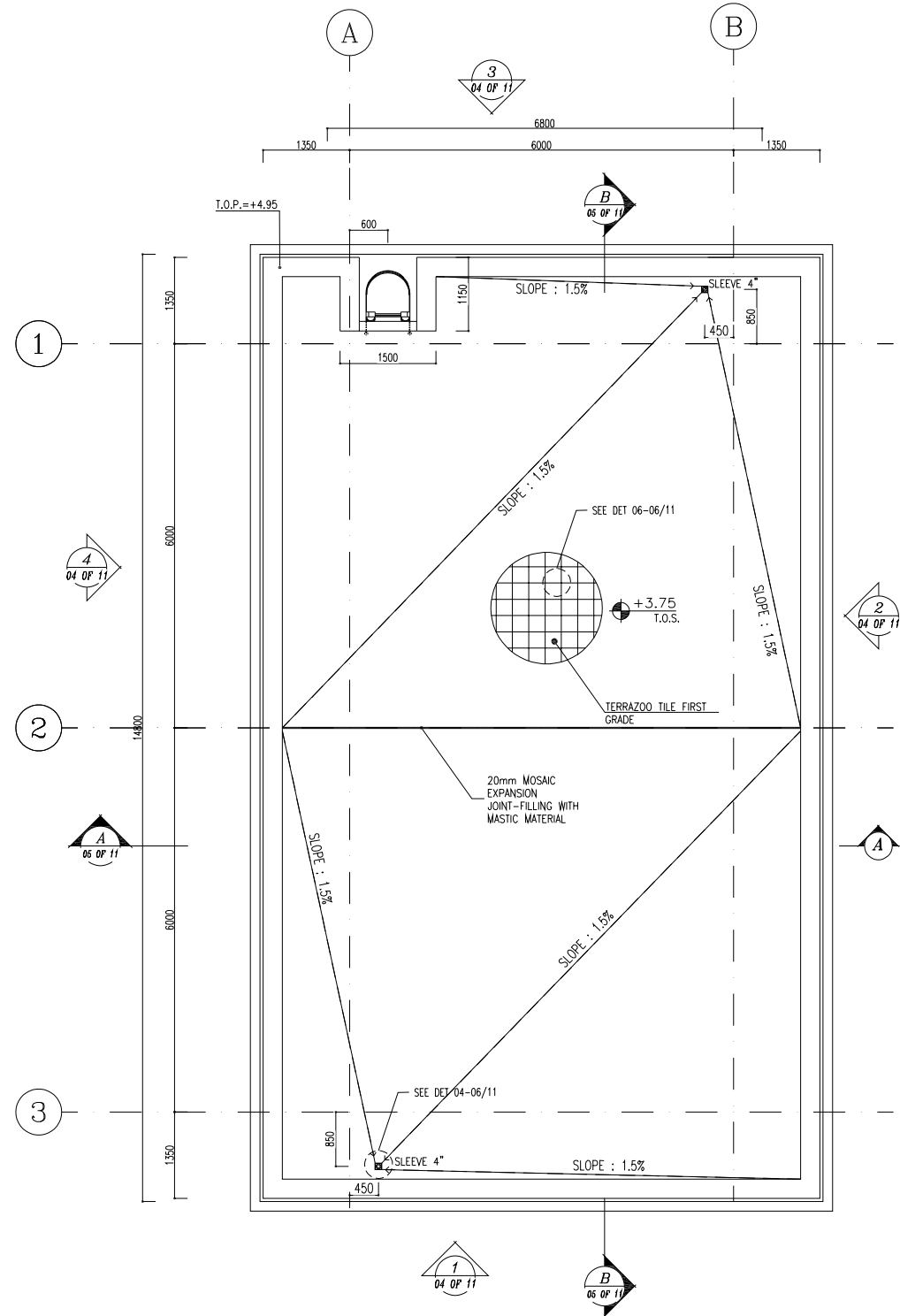
SC.1:50 2 ROOF PLAN
