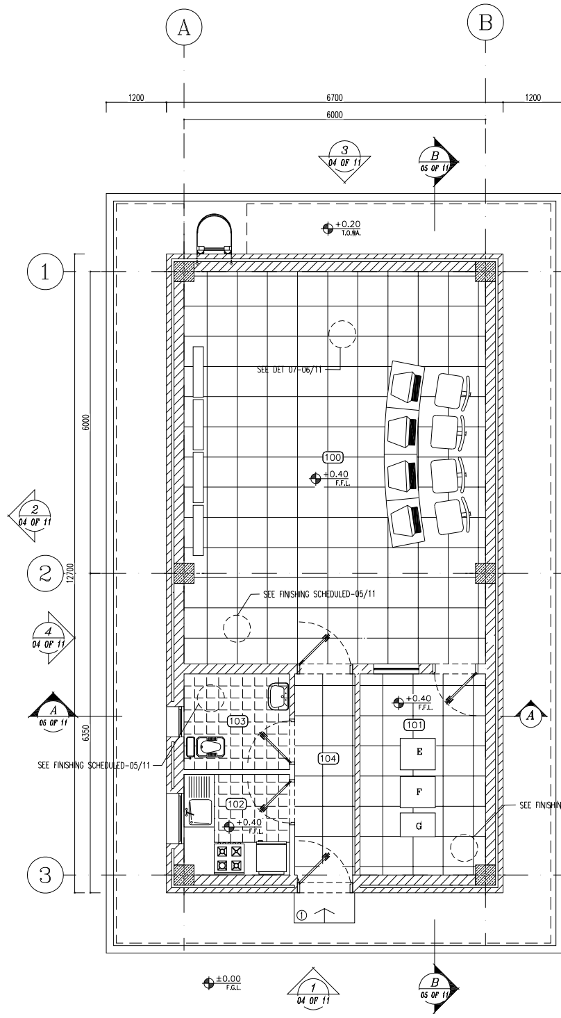
SC.1:50 3 FURNITURE PLAN
