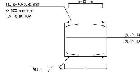
TYP. SECTION 2-2 Sc: 1:10
