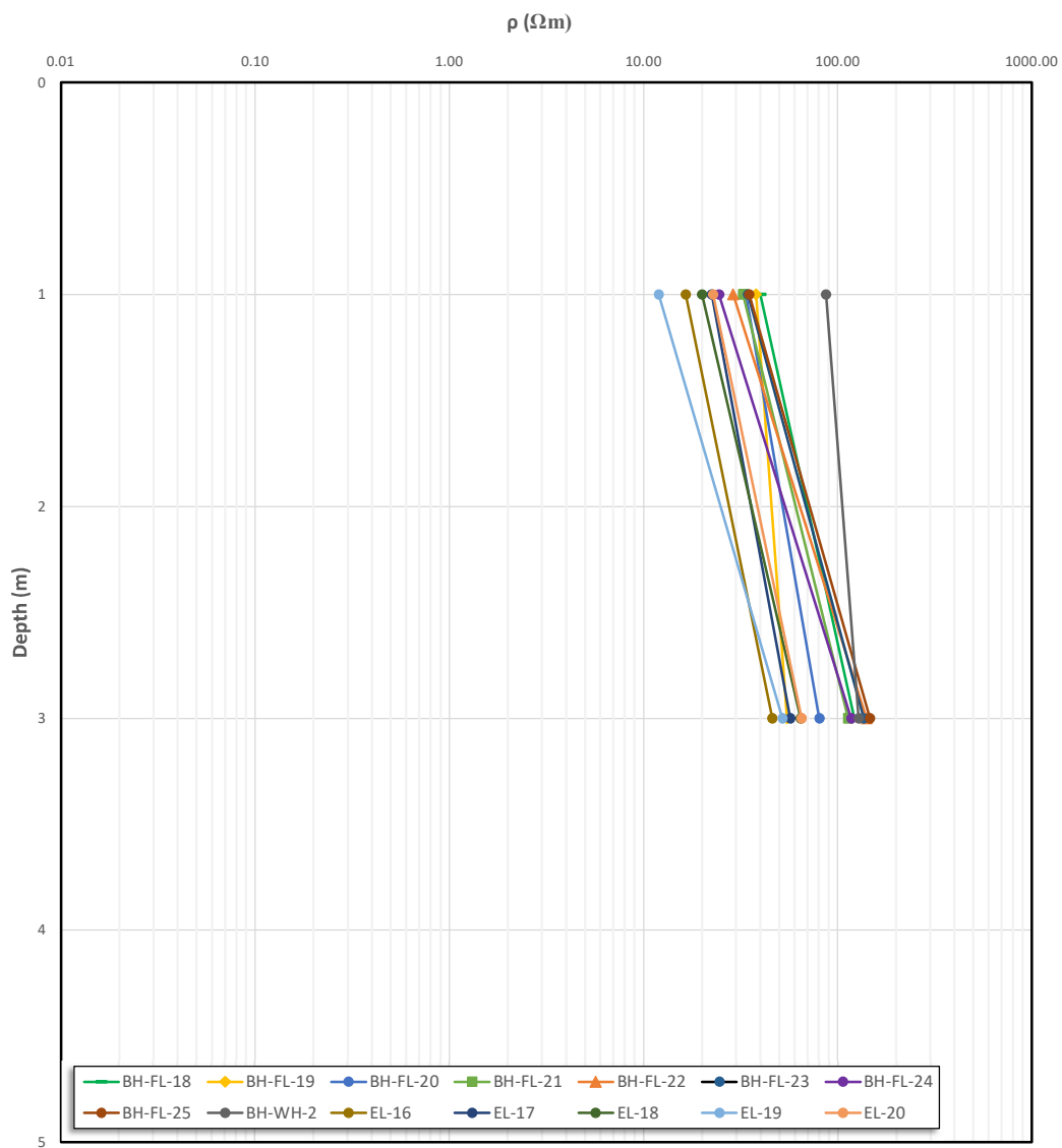
Variation of Apparant Electrical Resistivity in W-046
