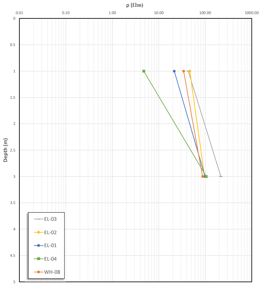
Variation of Apparant Electrical Resistivity in BK-5
