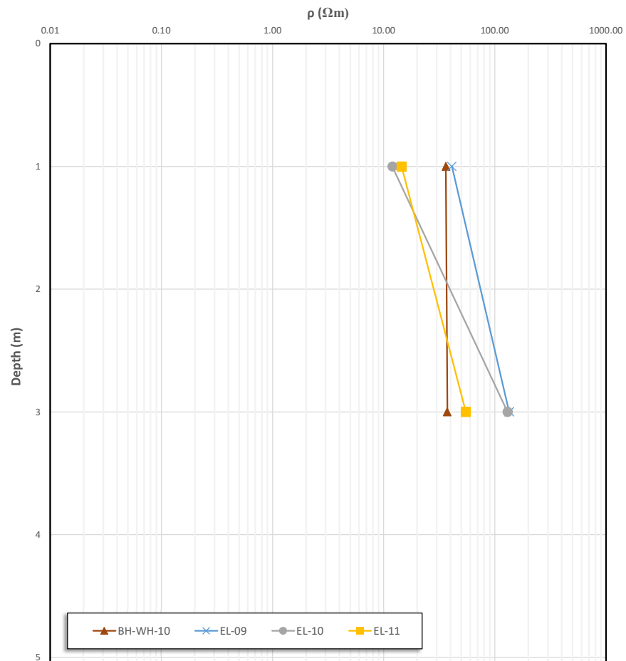
Variation of Apparant Electrical Resistivity in BK-14
