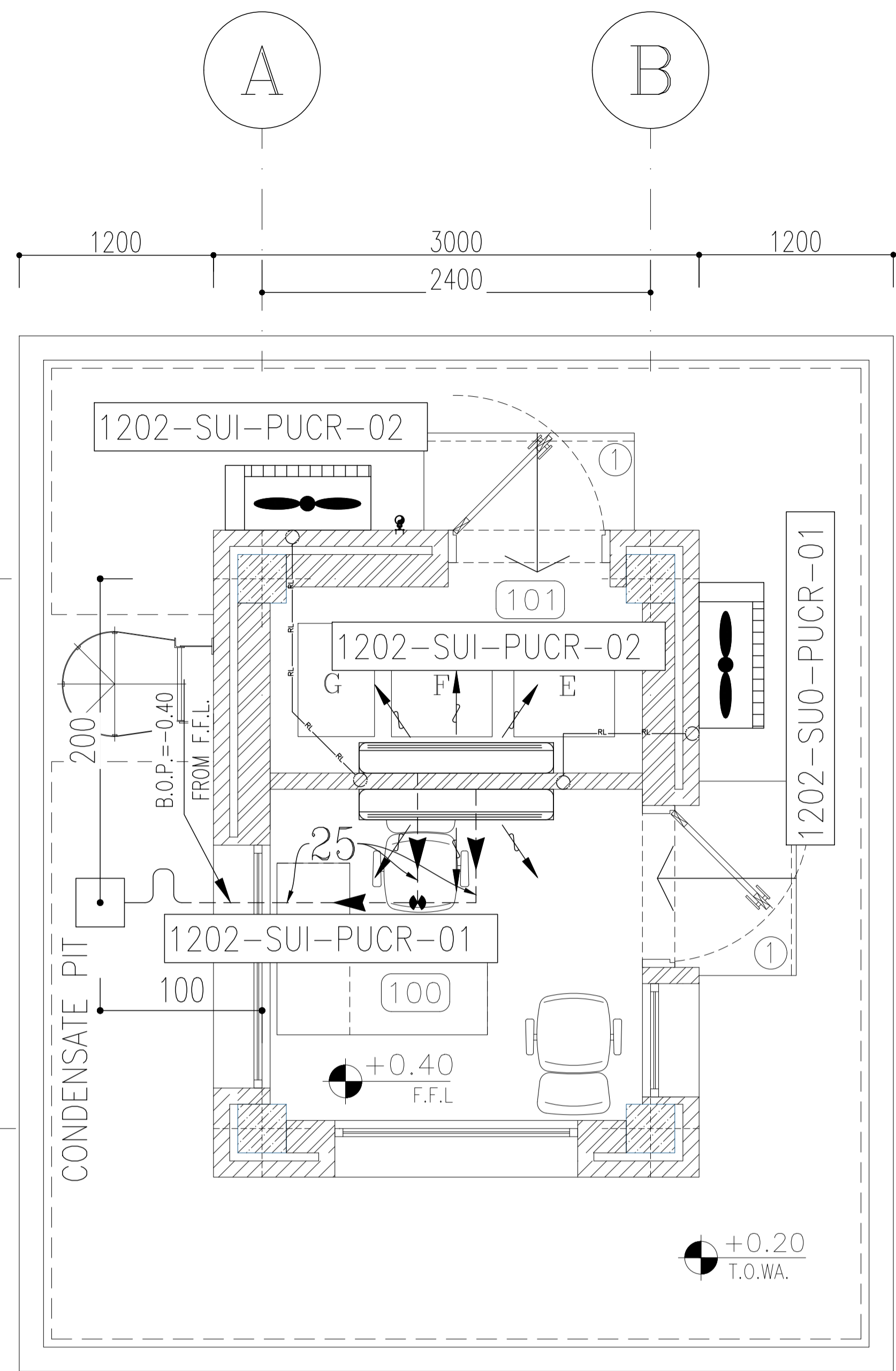
SC.1:25 1 FLOOR PLAN HVAC System Layout
