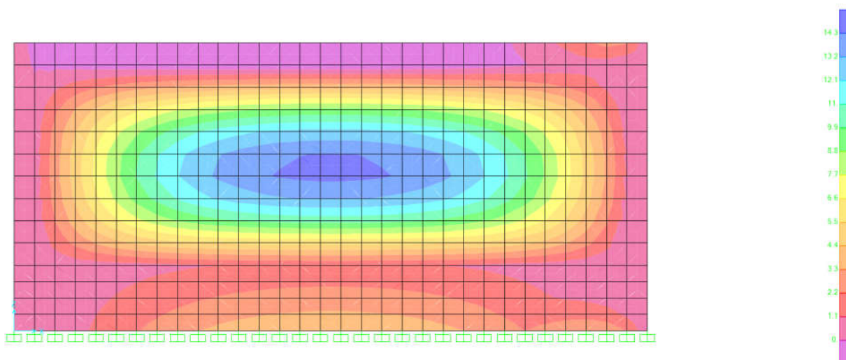
Figure 17- MAX M22 (ton-m)
