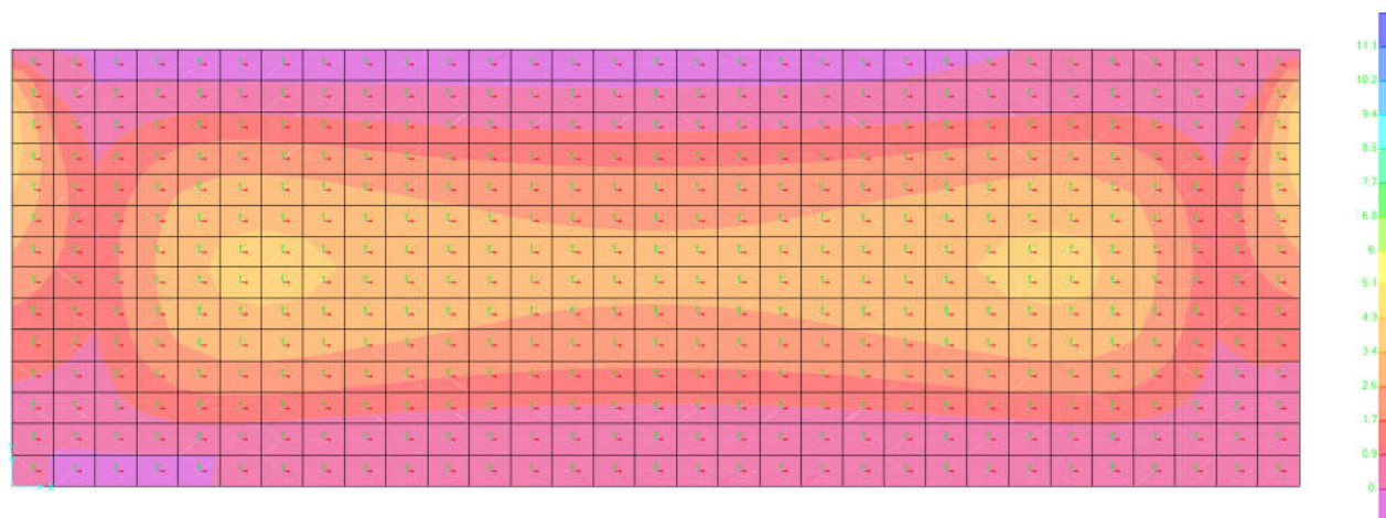
Figure 23- MAX M11 (ton-m)
