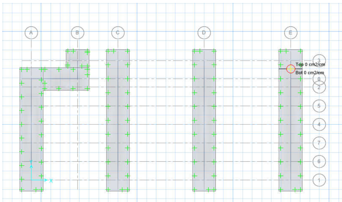
Figure 35- X DIRECTION REINFORCEMENT DESIGN
