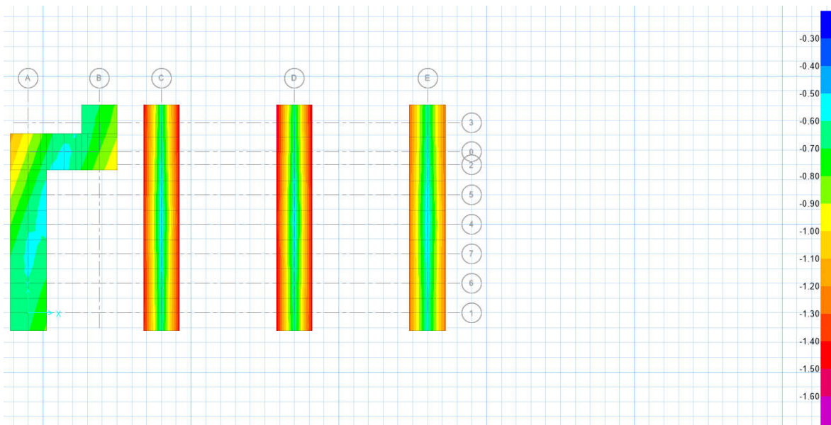
Figure 34- SOIL STRESS UNDER THE FOUNDATION
