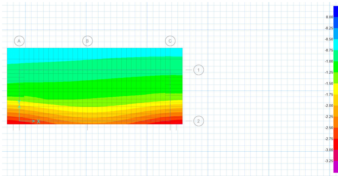
Figure 28- SOIL STRESS UNDER THE FOUNDATION
