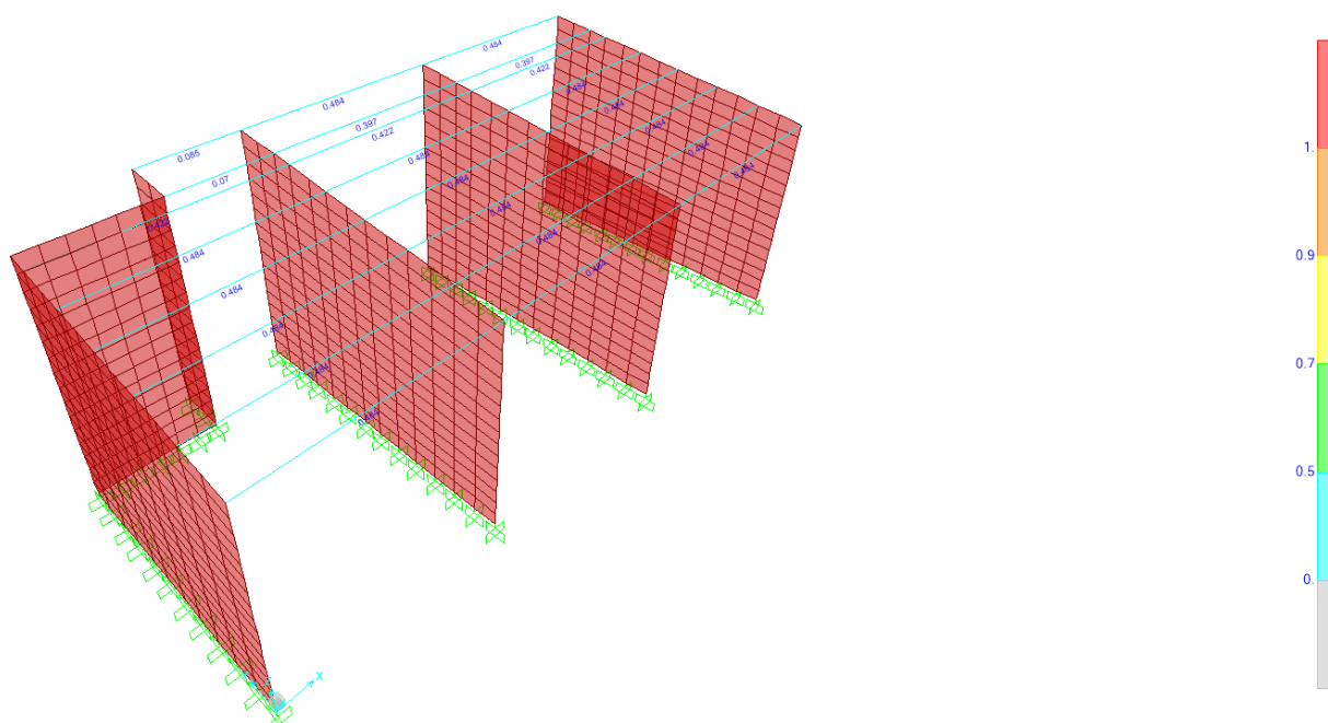
Figure 32- PURLIN DESIGN -Z180**2.5
