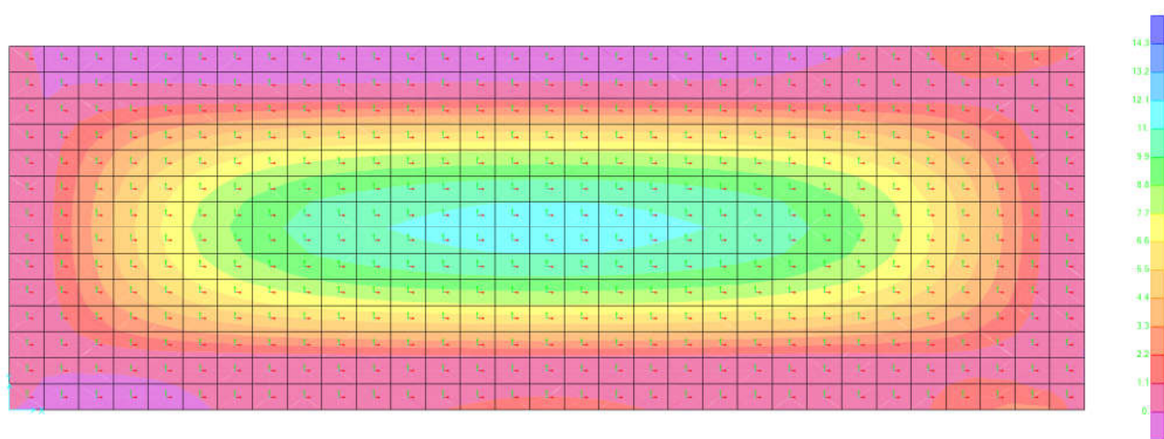
Figure 25- MAX M22 (ton-m)
