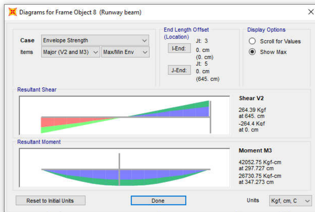
Figure 39- Moment 3-3 critical load combination on crane beam
