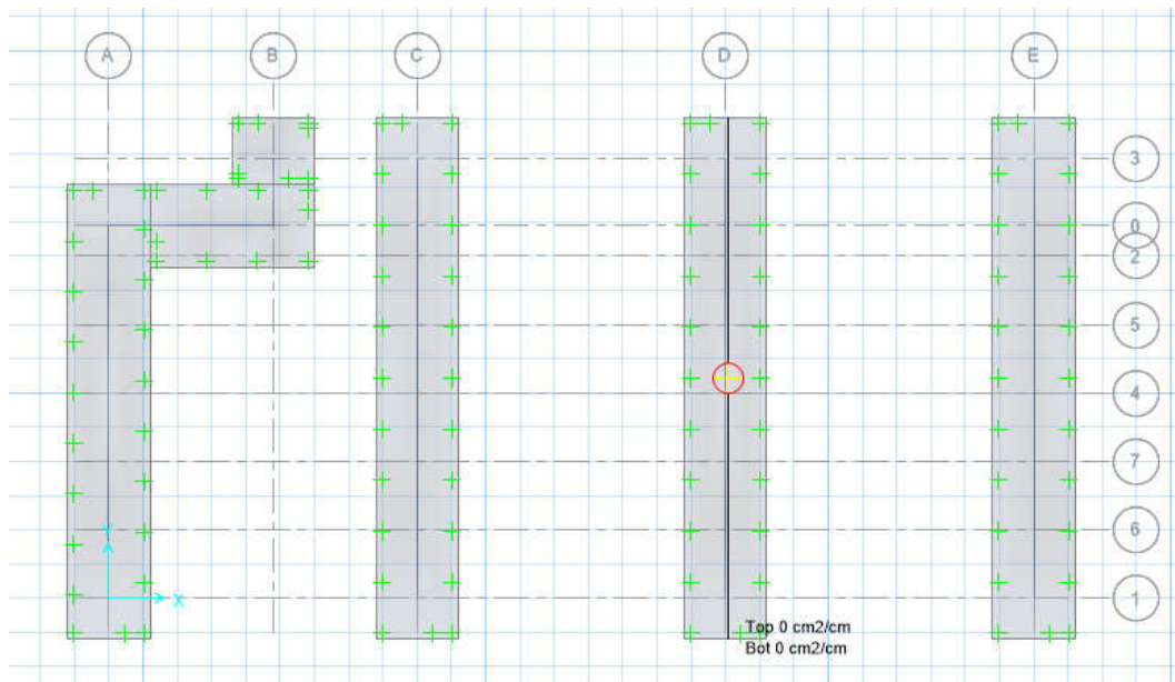
Figure 36- Y DIRECTION REINFORCEMENT DESIGN
