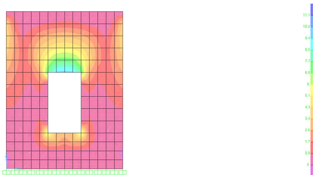
Figure 15- MAX M11 (ton-m)
