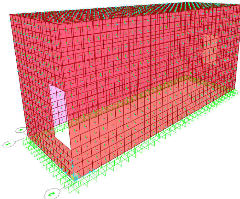
Figure 12- 3D MODEL OF CAPACITOR BANK AND CO2 ROOM
