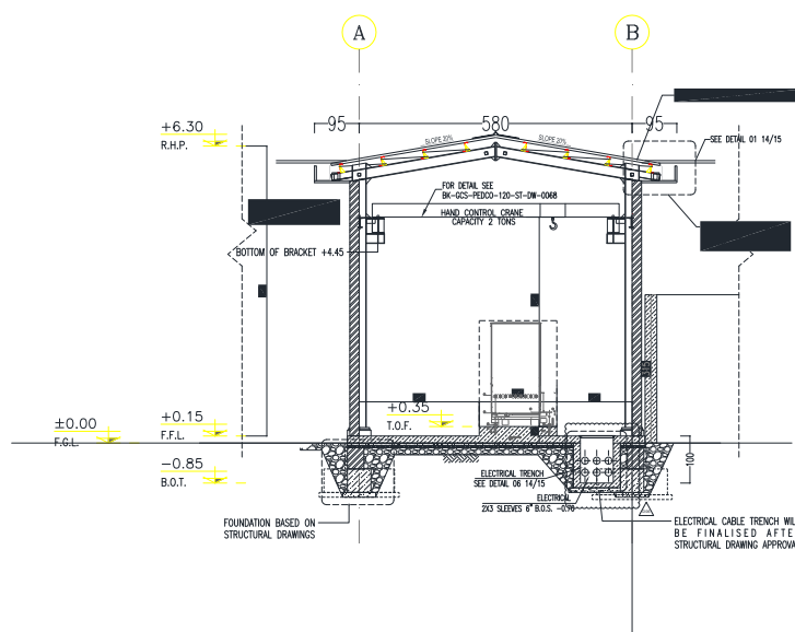
Figure 7 – SECTION E-E
