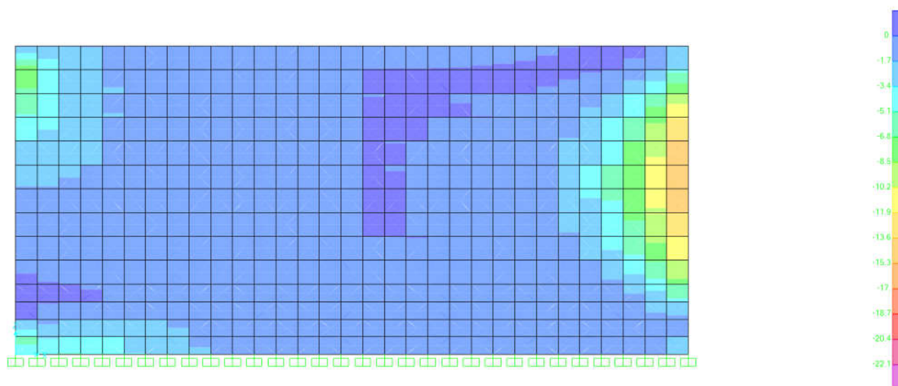
Figure 22- MIN V13 (ton)
