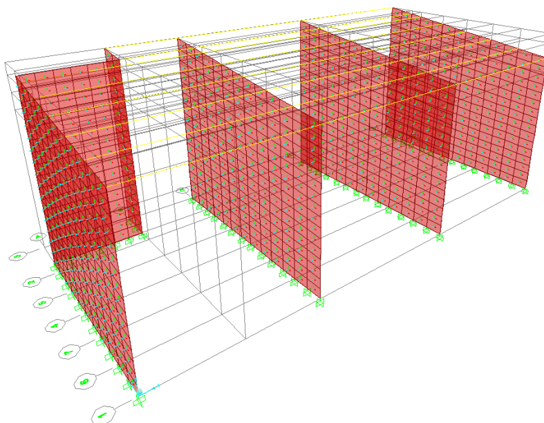
Figure 13- 3D MODEL OF TRANSFORMERS ROOM
