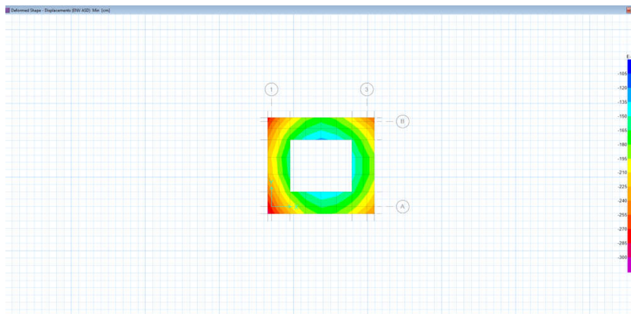
Figure 42- DEFORMED SHAPE (ENV COM - CM)
