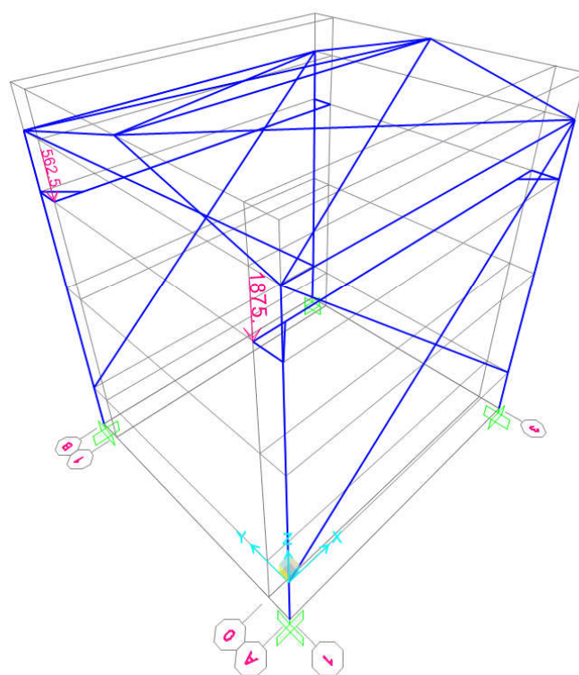
Figure 38- applied CRv load
