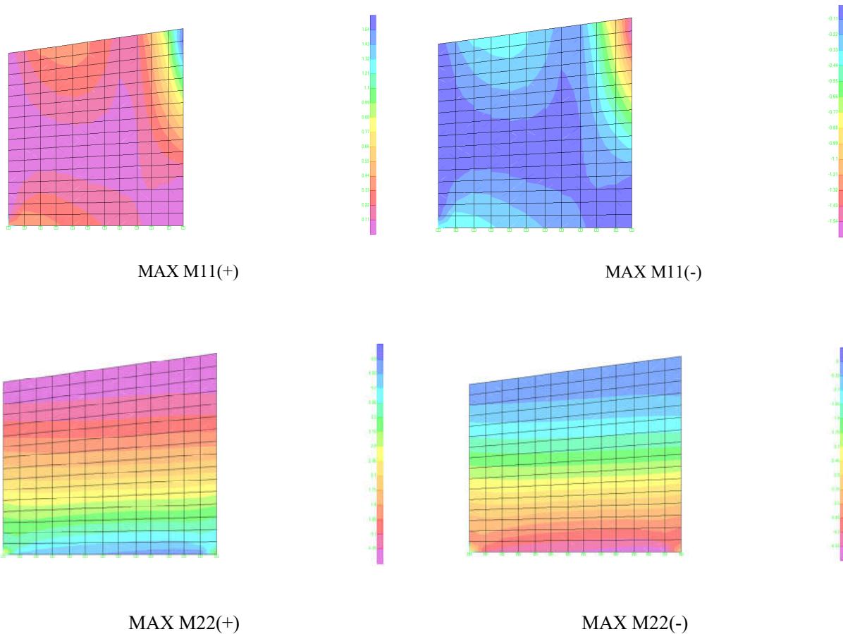
Figure 31- MAX WALL RESULTANT FORCES-ENVELOPE COMBO-(ton-m)
