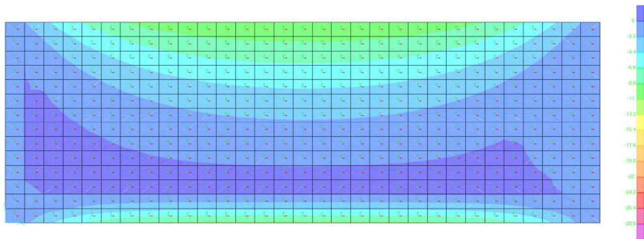
Figure 26- MINM22 (ton-m)
