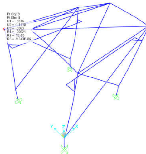
Figure 40- Deformed shape (maximum Drift critical Wx)
