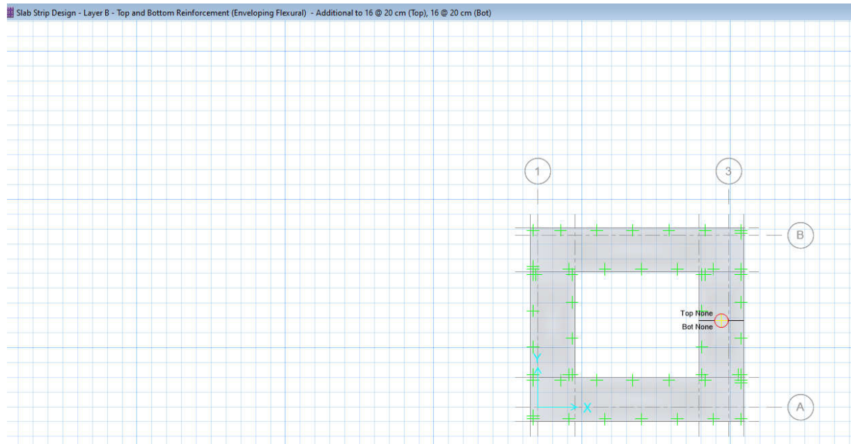
Figure 45- Y DIRECTION REINFORCEMENT DESIGN
