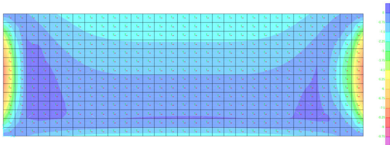
Figure 24- MIN M11 (ton-m)
