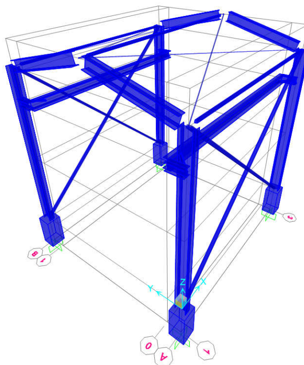
Figure 14- 3D MODEL OF DIESEL ROOM
