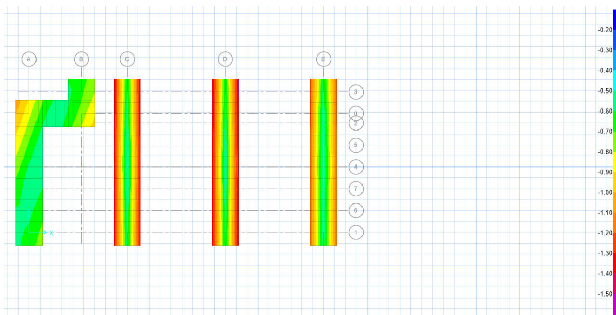
Figure 33- DEFORMED SHAPE (ENV COM - CM)
