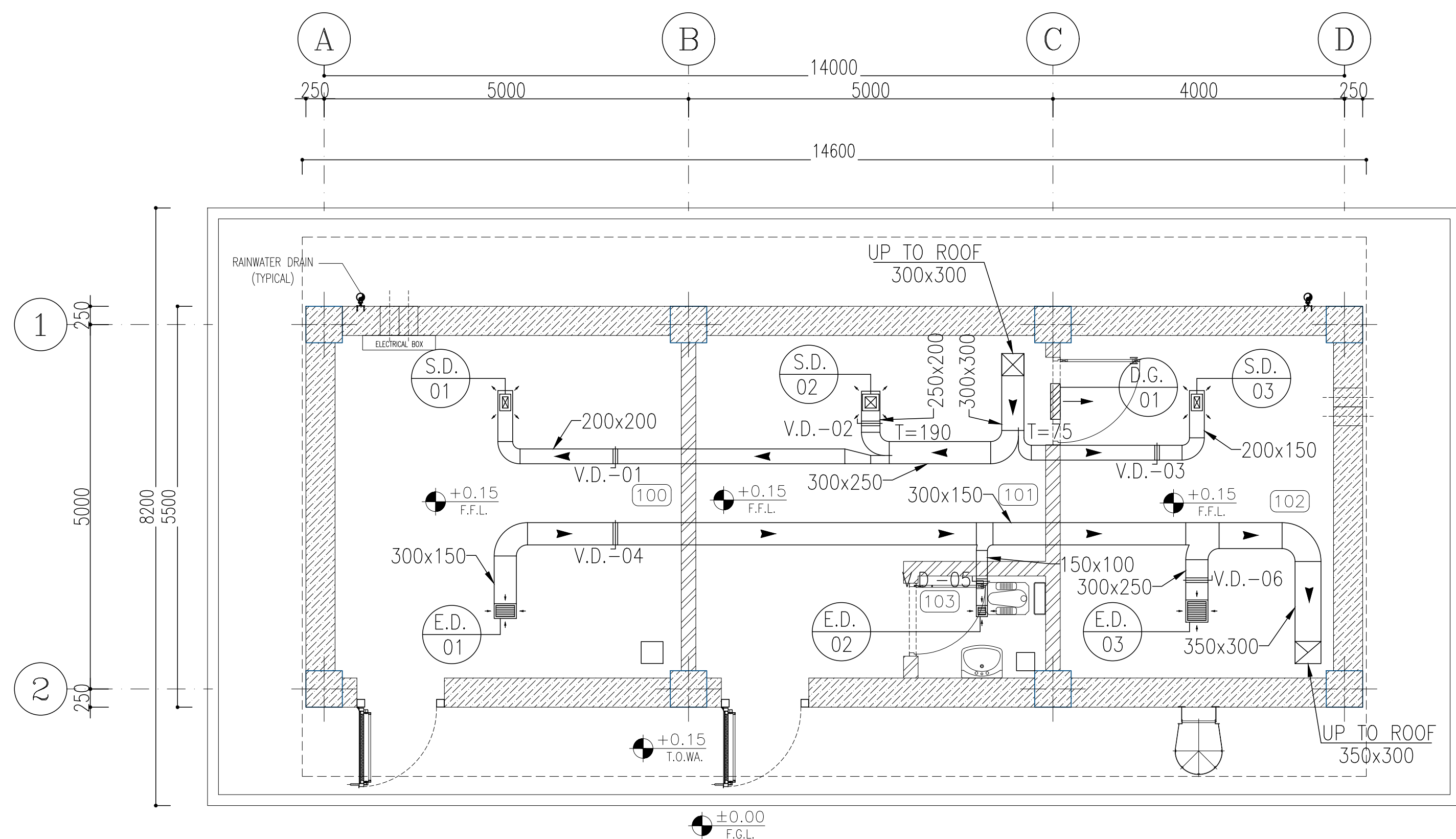
SC.1:50 1 FLOOR PLAN HVAC System Layout (HVAC Ducting)
