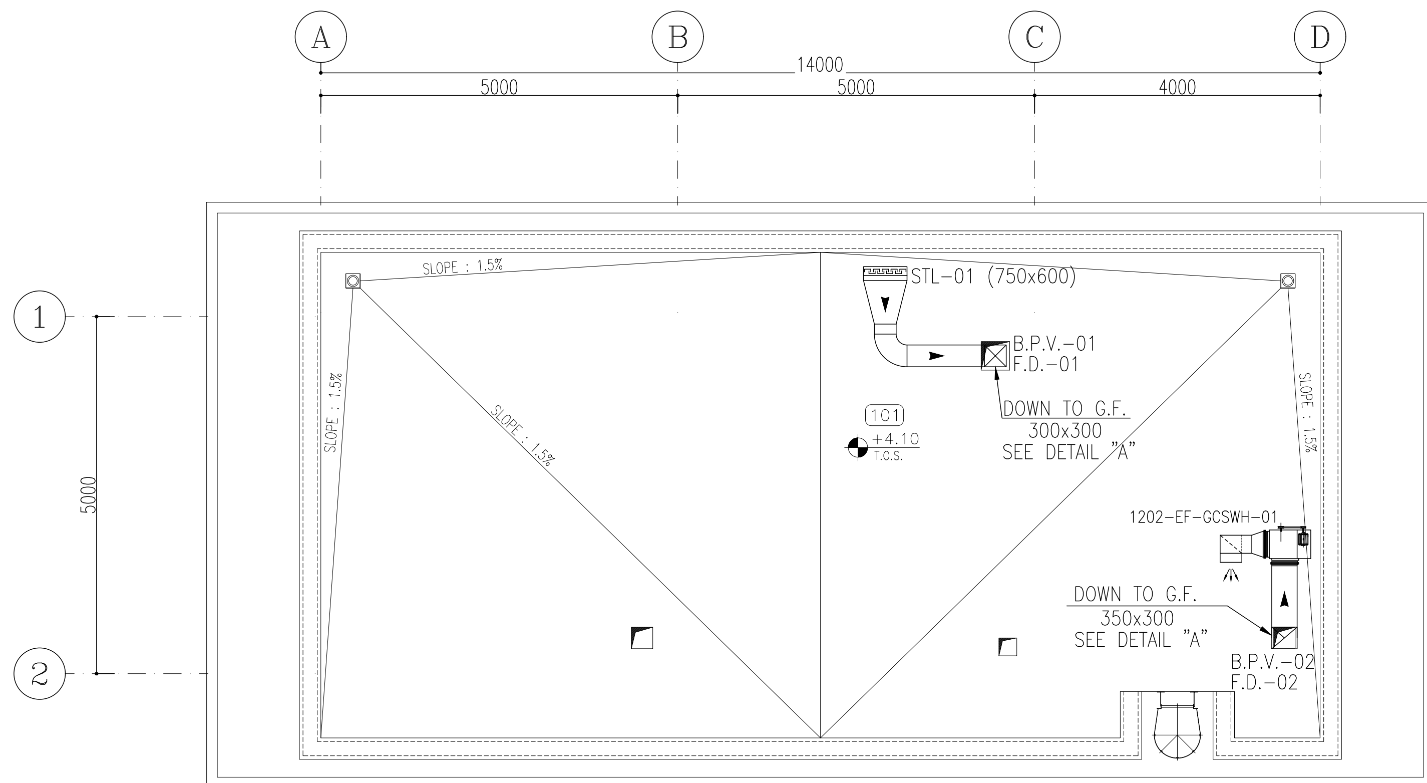
SC.1:50 1 FLOOR PLAN HVAC System Layout (HVAC Ducting)
