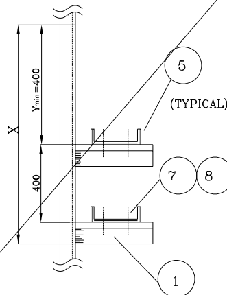
SUPPORT TO STEEL COLUMN
