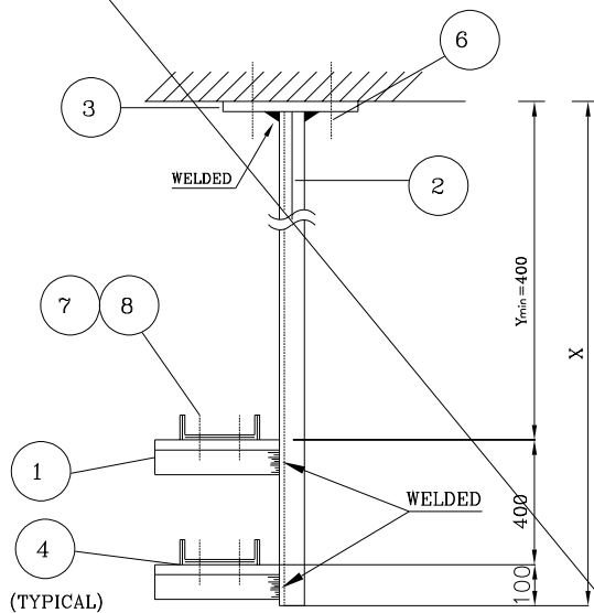
SUPPORT TO STEEL STRUCTURE
