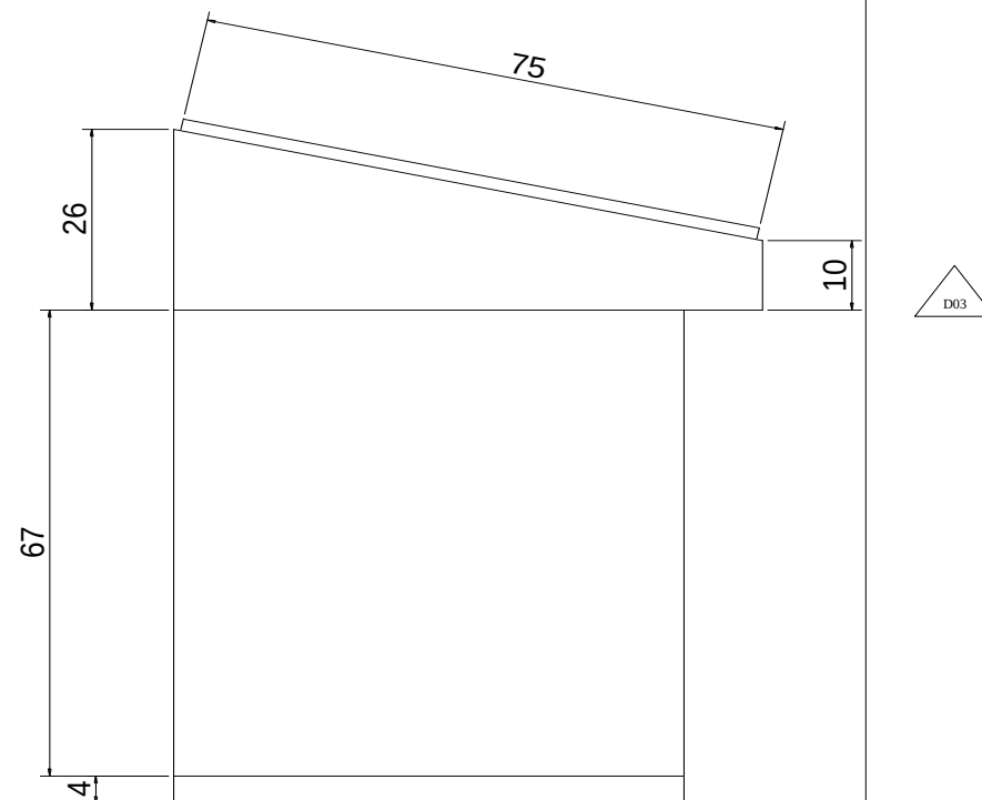
SIDE VIEW OF PANEL (TO BE FINALIZED BY VENDOR) ESD CONSOLE AND F&G CONSOLE HAVE SAME SEDIGN
