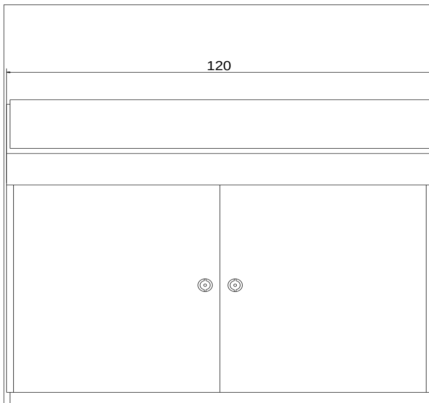
FRONT VIEW OF PANEL (TO BE FINALIZED BY VENDOR) ESD CONSOLE AND F&G CONSOLE HAVE SAME SEDIGN
