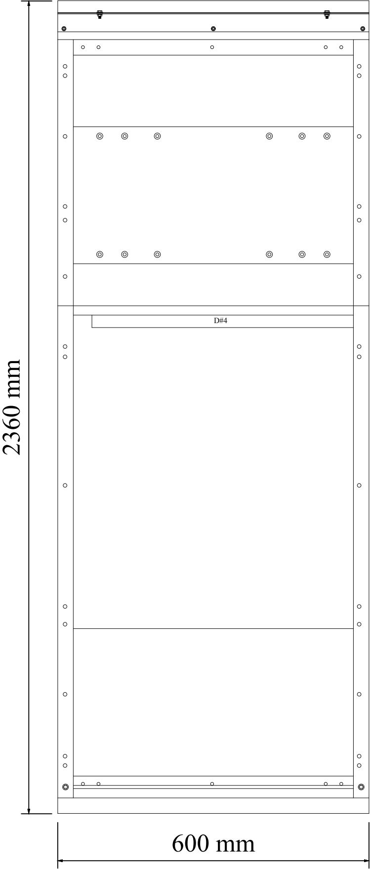
Back View(Door Layout)
