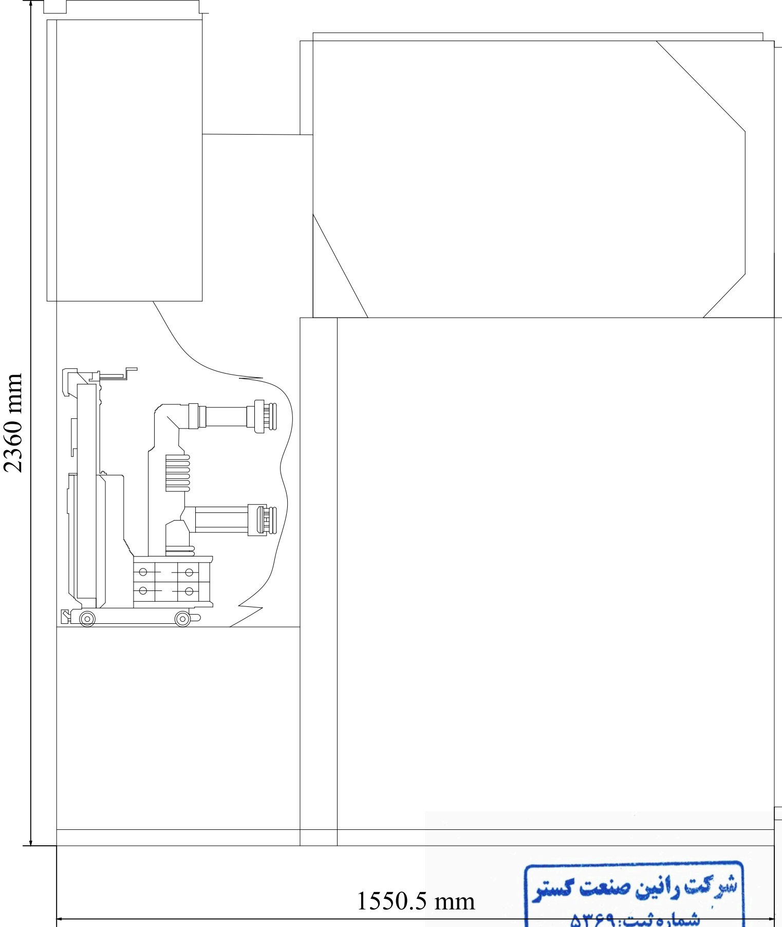
Side View(Depth Layout)
