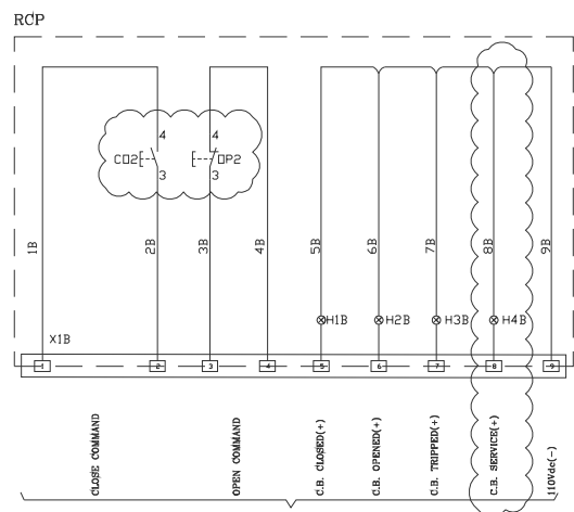
11KV CIRCUIT BREAKER GCS-TR-002, TRANSFORMER-002 11/0.42 KV
