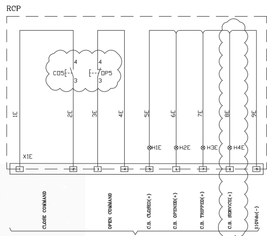
11KV SPARE CIRCUIT BREAKER
