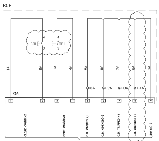
11KV CIRCUIT BREAKER GCS-TR-001, TRANSFORMER-001 11/0.42 KV
