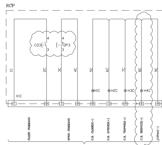
11KV CIRCUIT BREAKER GCS-TR-003, TRANSFORMER-003 11/3.3 KV
